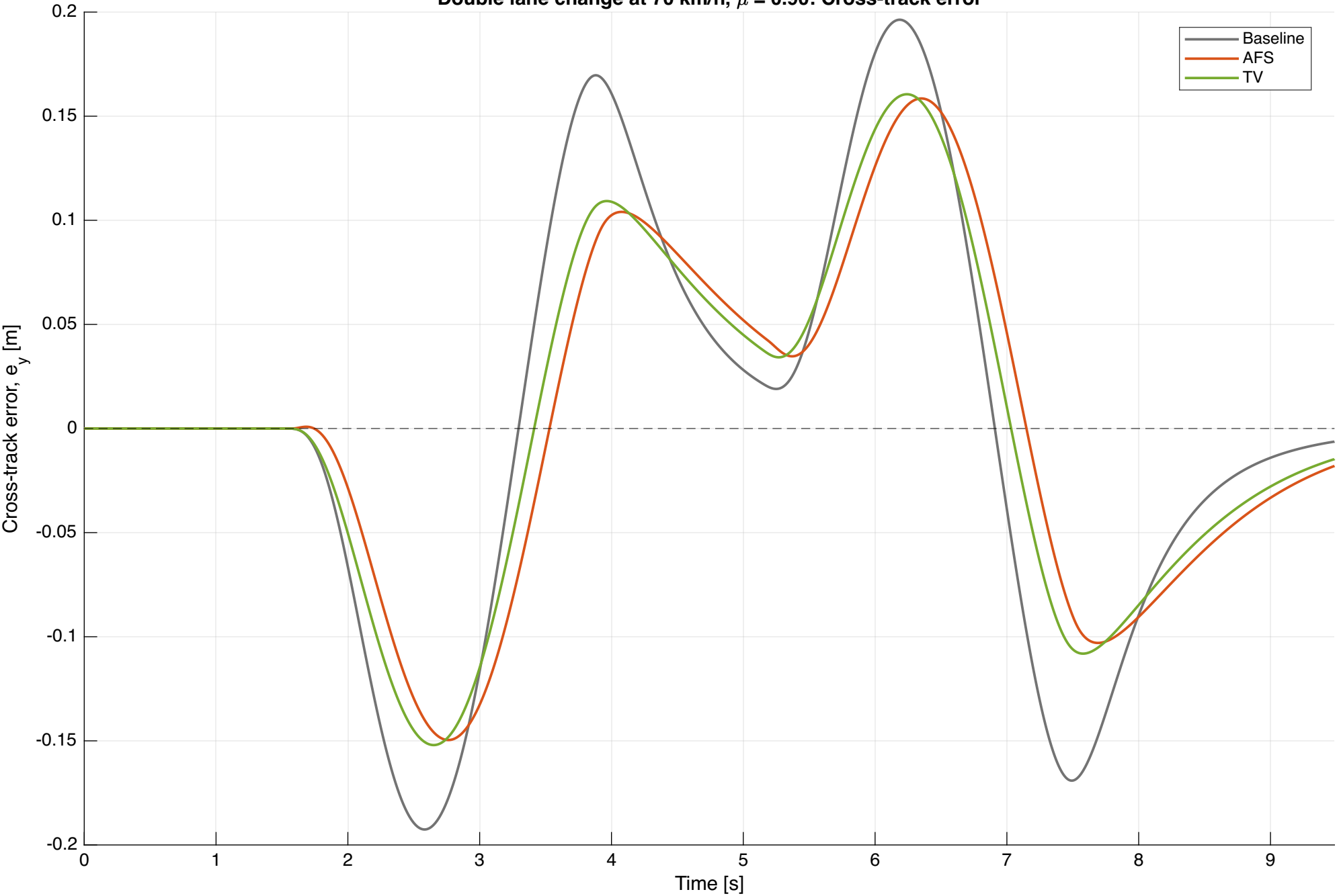
Double lane change at 70 km/h, \mu = 0.90 : Cross-track error
