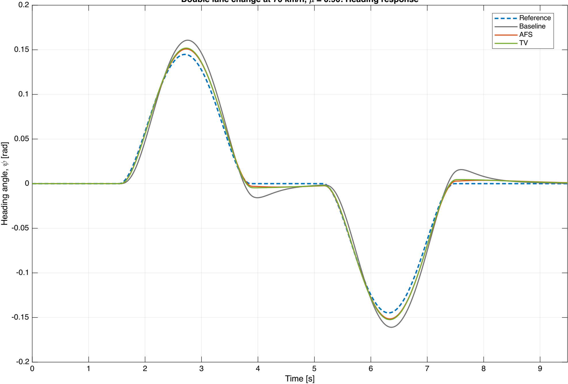
Double lane change at 70 km/h, \mu = 0.90 : Heading response
