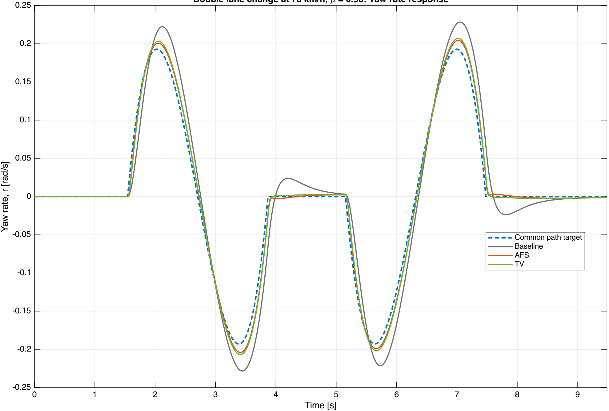
Double lane change at 70 km/h, \mu = 0.90 : Yaw-rate response
