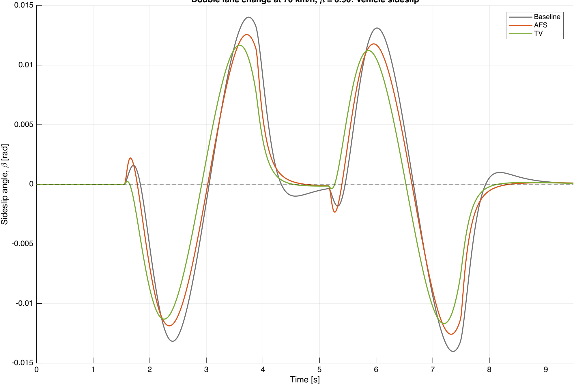
Double lane change at 70 km/h, \mu = 0.90 : Vehicle sideslip
