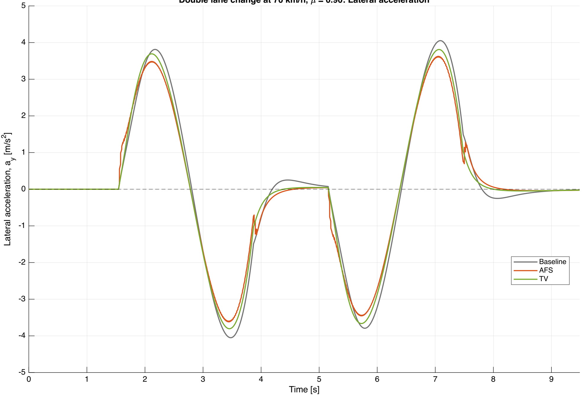
Double lane change at 70 km/h, \mu = 0.90 : Lateral acceleration
