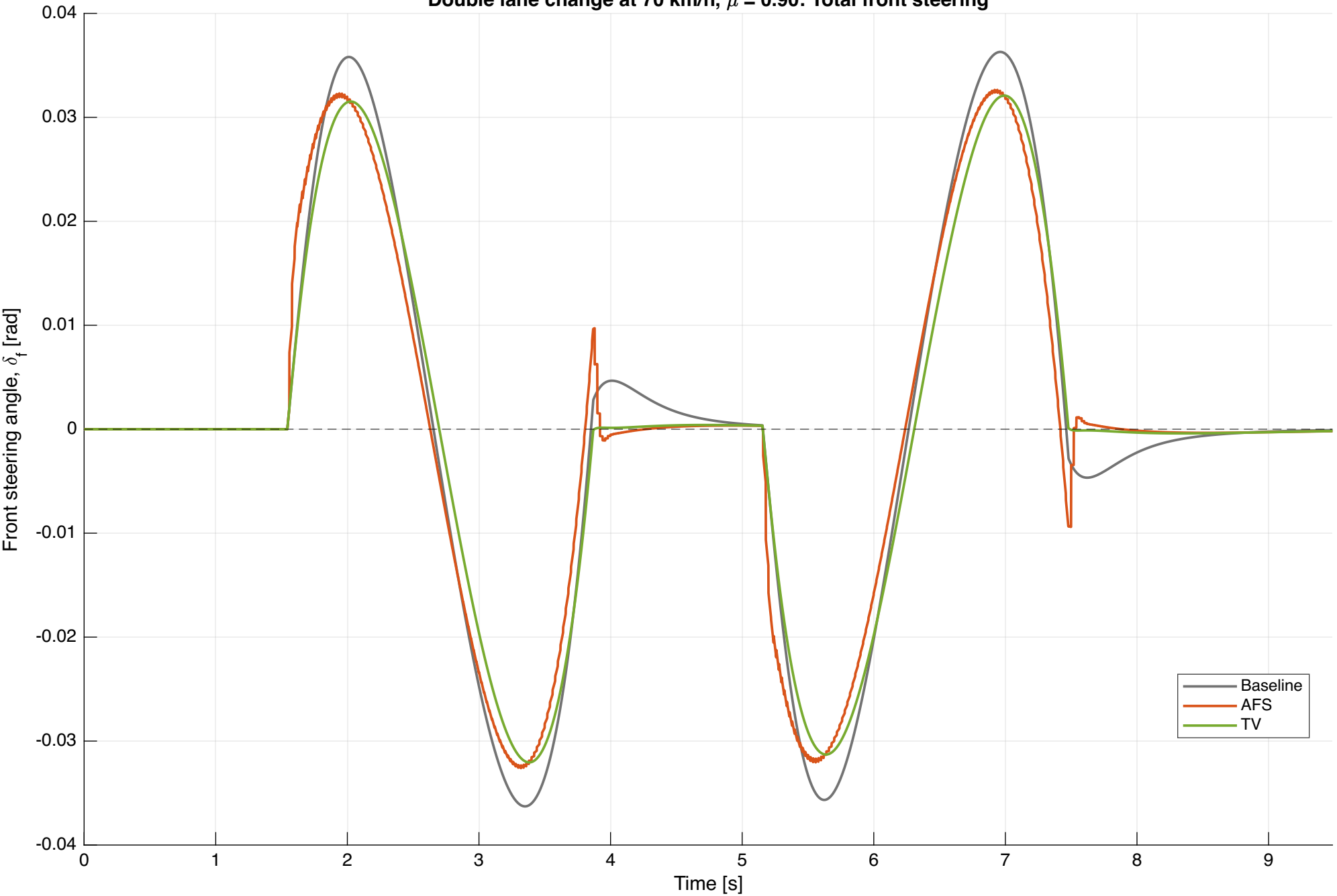
Double lane change at 70 km/h, \mu = 0.90 : Total front steering
