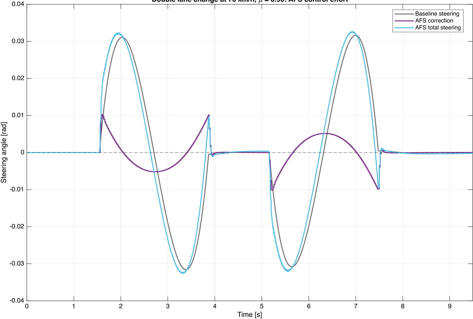
Double lane change at 70 km/h, \mu = 0.90 : AFS control effort
