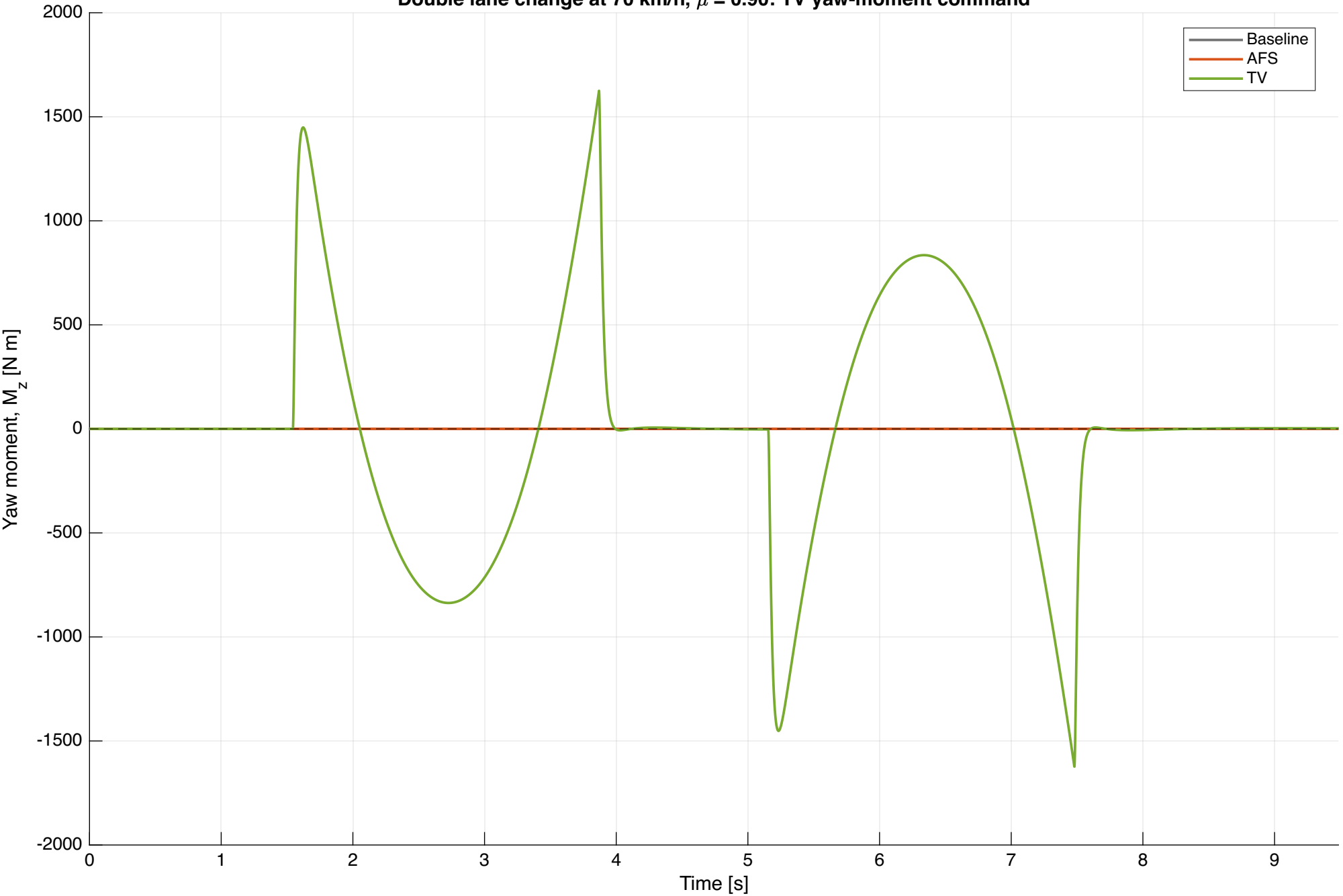
Double lane change at 70 km/h, \mu = 0.90 : TV yaw-moment command
