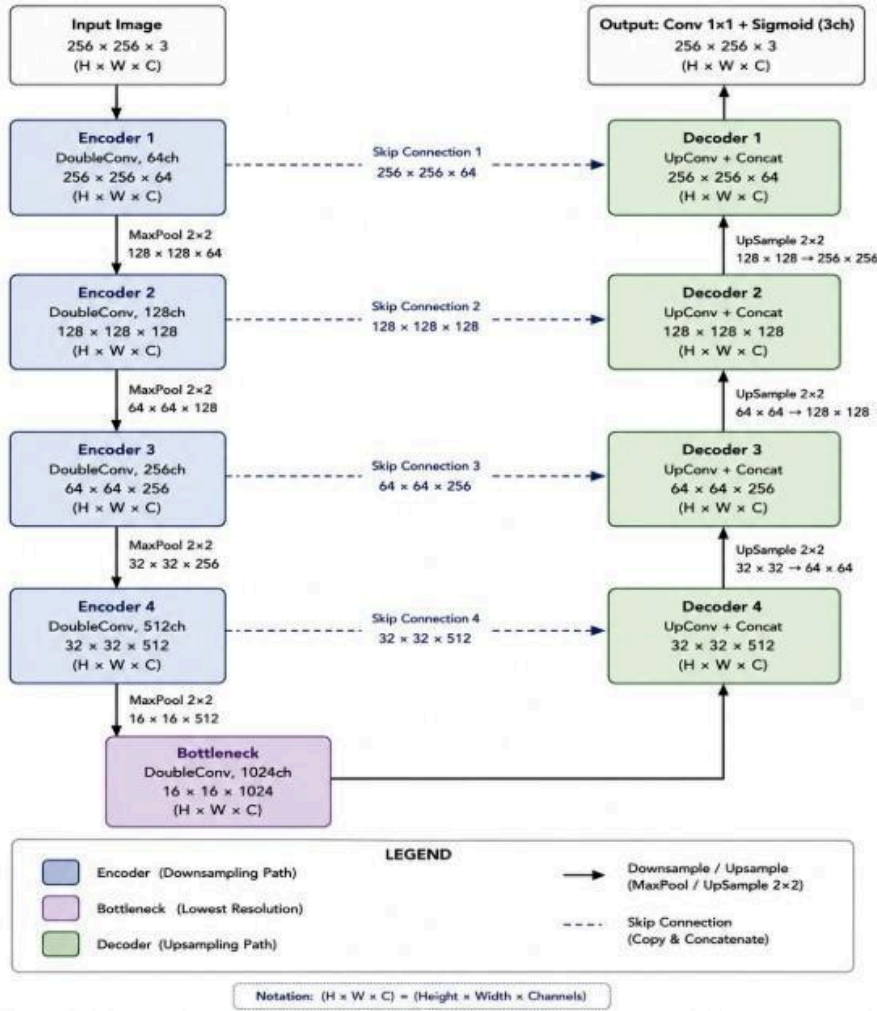
Fig.2.1: In the Baseline U-Net architecture, every encoder block, the bottleneck, and every decoder block employ standard DoubleConv operations without attention mechanisms. Skip connections link each encoder stage to its corresponding decoder stage, enabling the preservation of fine spatial details during image reconstruction.
