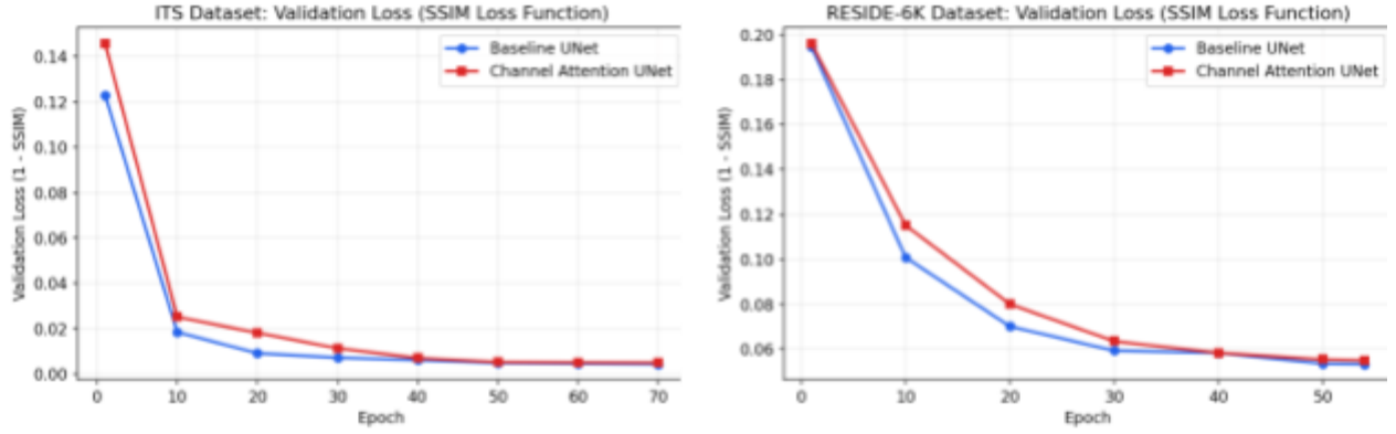
Fig.3.1: Validation-loss curves (SSIM loss), ITS (left): Baseline (blue) vs. Channel Attention (red); RESIDE-6K (right): Baseline (blue) vs. Channel Attention (red).
