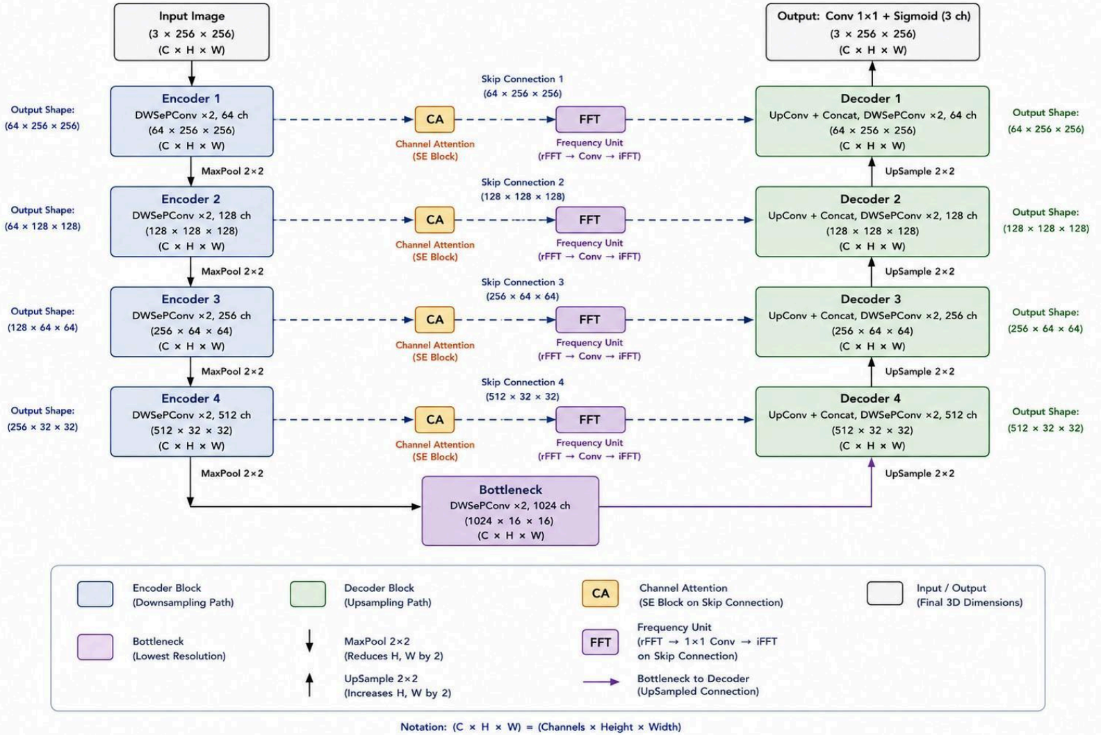
Fig.2.5: Depthwise + Skip Channel Attention + FFT U-Net architecture. The encoder, bottleneck, and decoder employ depthwise separable convolutions, while each skip connection is refined by a Channel Attention (SE) block followed by a frequency-domain processing unit. The Frequency Unit applies a two-dimensional real Fast Fourier Transform (rFFT2), performs learnable filtering on the real and imaginary frequency components using 1 \times 1 convolutions, reconstructs the complex representation, and returns to the spatial domain via the inverse real Fast Fourier Transform (iFFT2). The frequency-refined skip features are then concatenated with the decoder features to combine adaptive channel weighting with global frequency-domain refinement.
