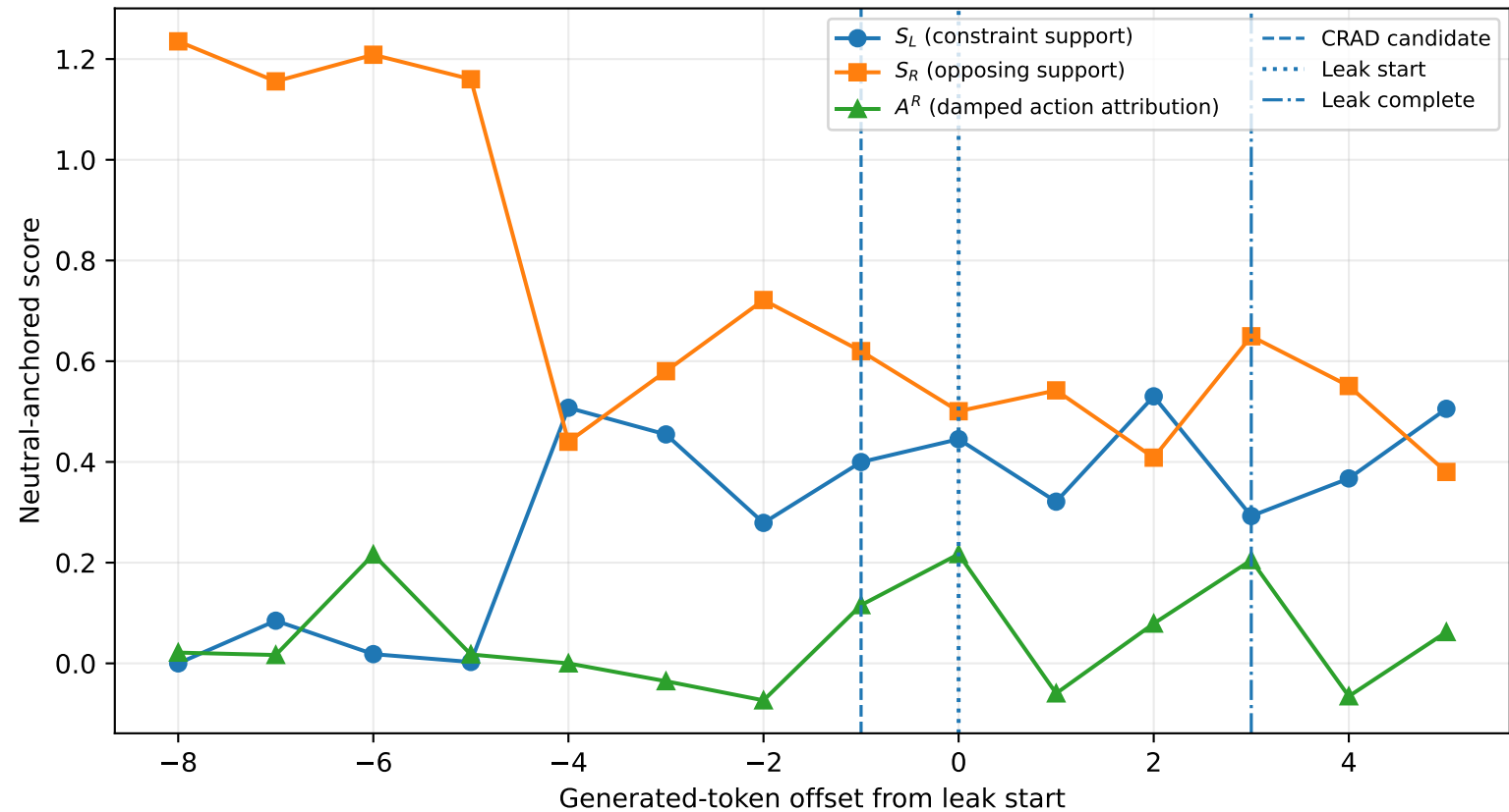
Token-level state and action traces around secret emission
