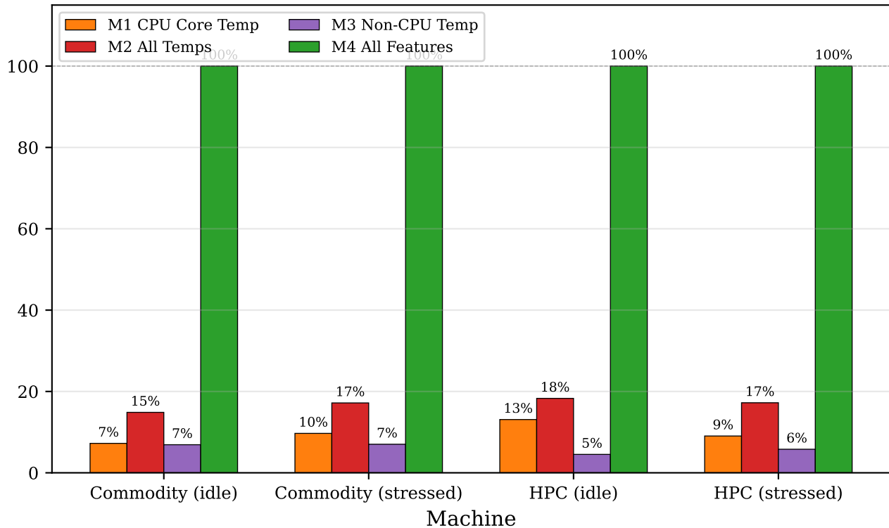
% of Total SHAP Importance
