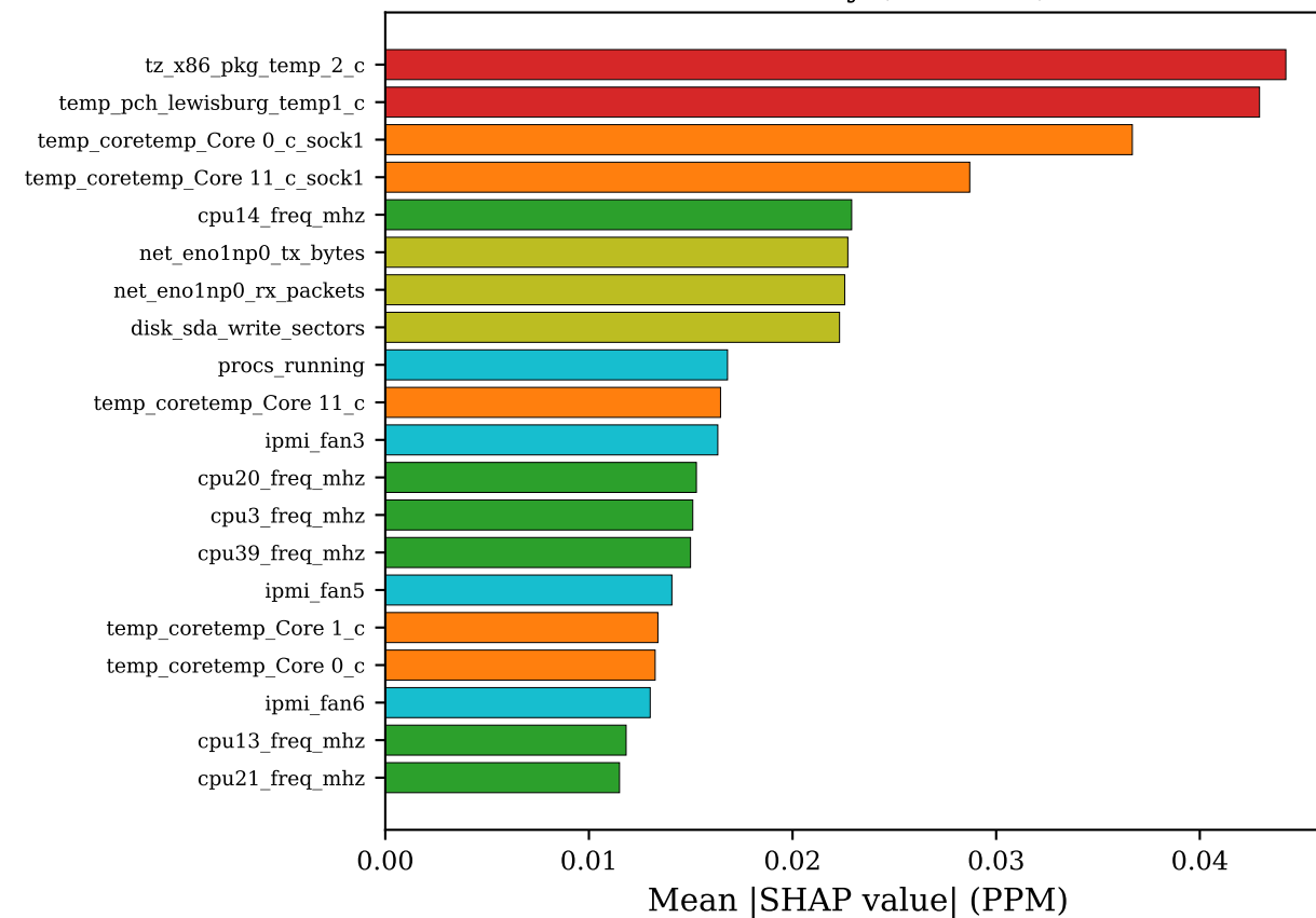
HPC (stressed)
