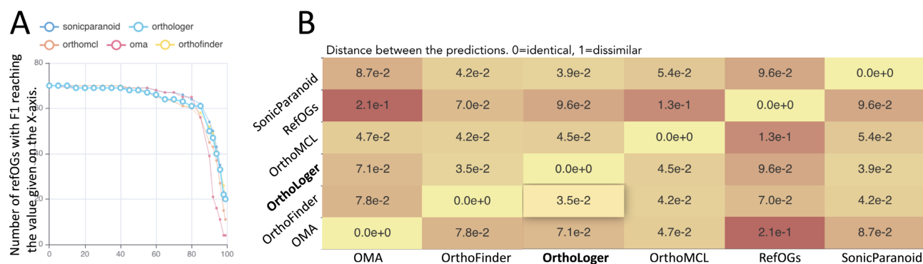
Figure 2. Benchmark ( https://lemortho.ezlab.org/refogs ) of the OrthoLogger software on refOGs. (A) The distribution of the F1 metric over refOGs shows that for the majority of refOGs F1 > 80%. (B) Concordance on ‘Variation of Information’ between the methods and RefOGs. The lower values indicate more similar classifications.
