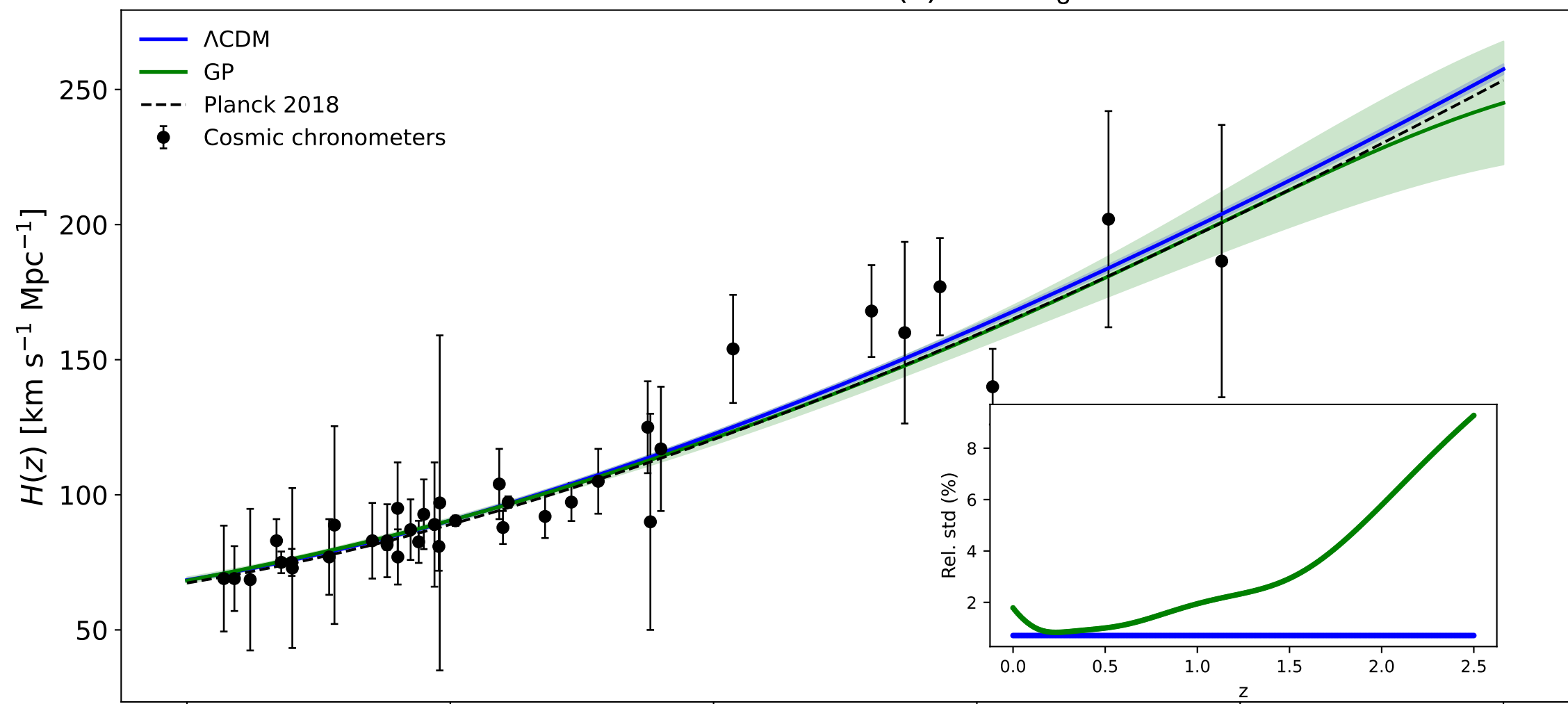
Constraints on H(z) and f\sigma_8
