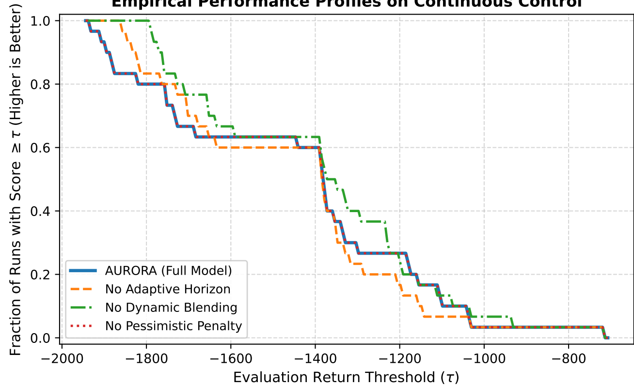
Empirical Performance Profiles on Continuous Control
