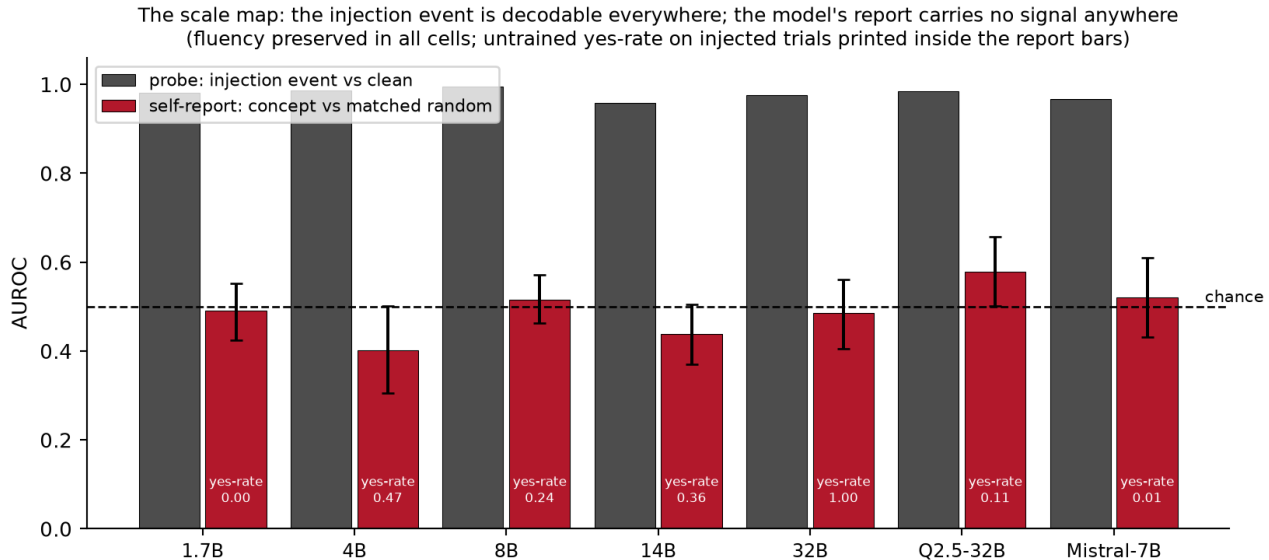
Figure 1: The scale map. The injection event is decodable from the final-layer state everywhere (grey); the model’s spontaneous report carries no signal anywhere (red), with untrained yes-rates printed in the bars. Every cell preserves output fluency.
