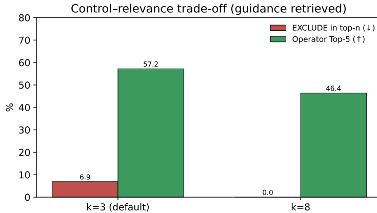
Figure 3: Control–relevance trade-off: retrieving more guidance ( k_{\text{guidance}}=8 ) achieves full EXCLUDE enforcement but lowers operator Top-5 accuracy.
