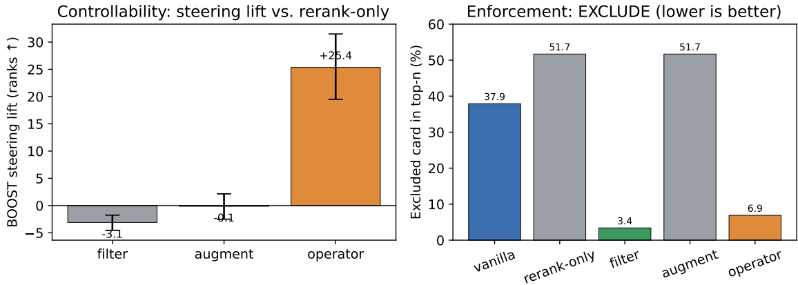
Figure 2: Left: BOOST steering lift over rerank-only with 95% CIs — only the operator’s excludes zero; filter and augment do not. Right: rate at which an EXCLUDE target still appears in the top- n (filter and operator both drive it down; augment does nothing).
