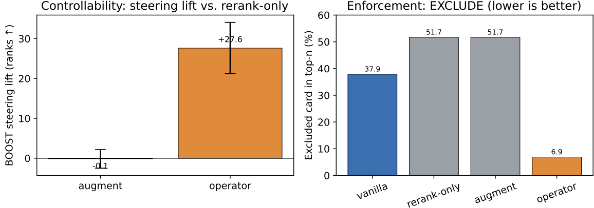
Figure 2: Left: BOOST steering lift over rerank-only with 95% CIs — the operator’s excludes zero, augment’s does not. Right: rate at which an EXCLUDE target still appears in the top- n (the operator drives it down; augment does nothing).
