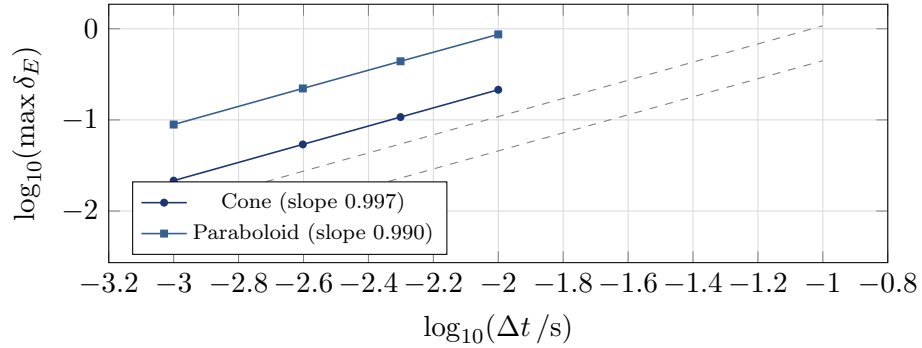
Figure 5: Log-log plot of maximum energy drift vs. time step for bounded runs. Slopes near unity confirm first-order Euler scaling (Table 3).
