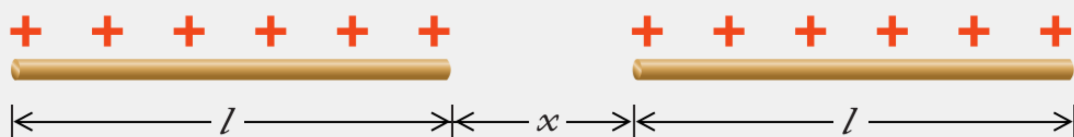
FIGURE 25.46 Two aligned charged rods.
