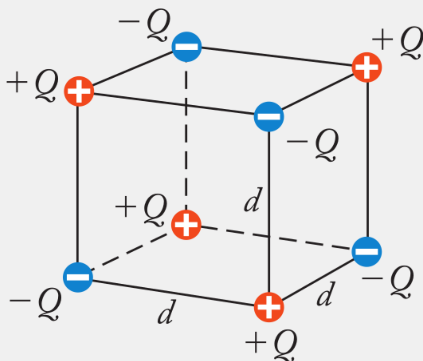
FIGURE 25.40 Point charges at the corners of a cube.
