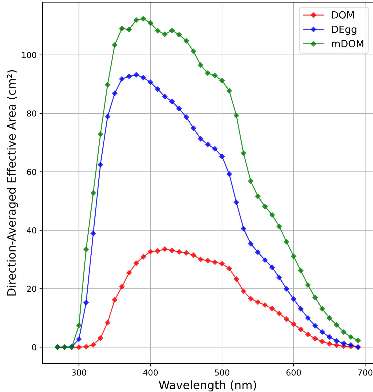
Effective Area vs Wavelength
