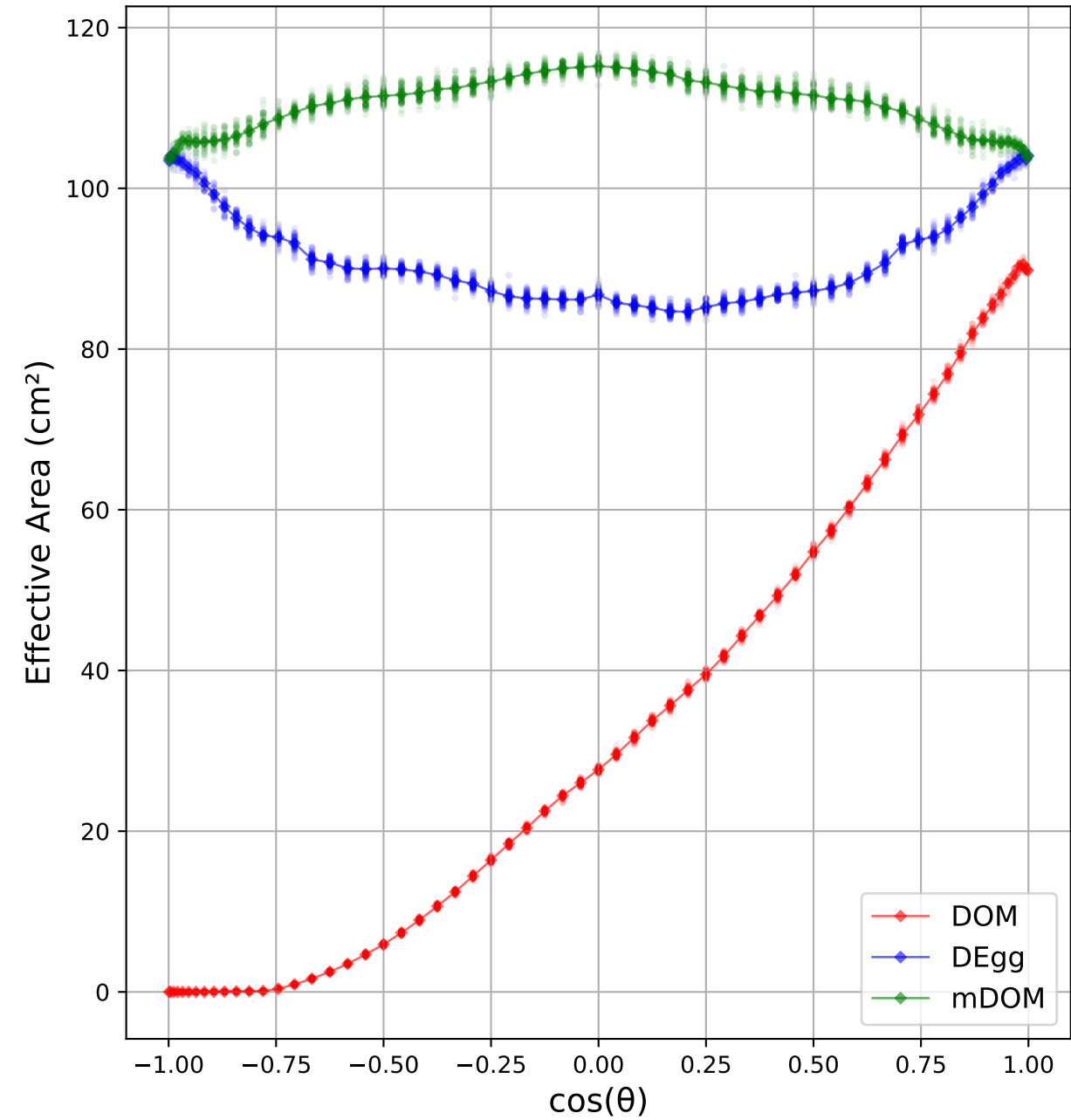
Effective Area vs \cos(\theta) at 400nm
