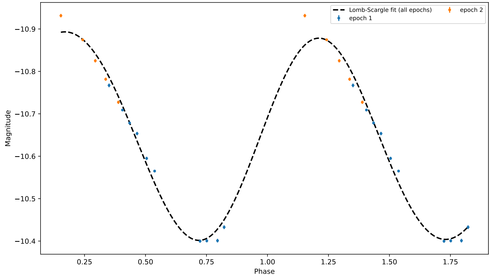
Lomb-Scargle Fit (nterms=3) - 0.3078801283505586 days = 7h 23m 20.843s
