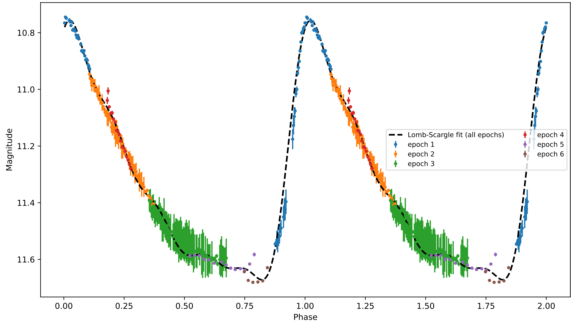
Lomb-Scargle Fit (nterms=5) - 0.46808109934410064 days
