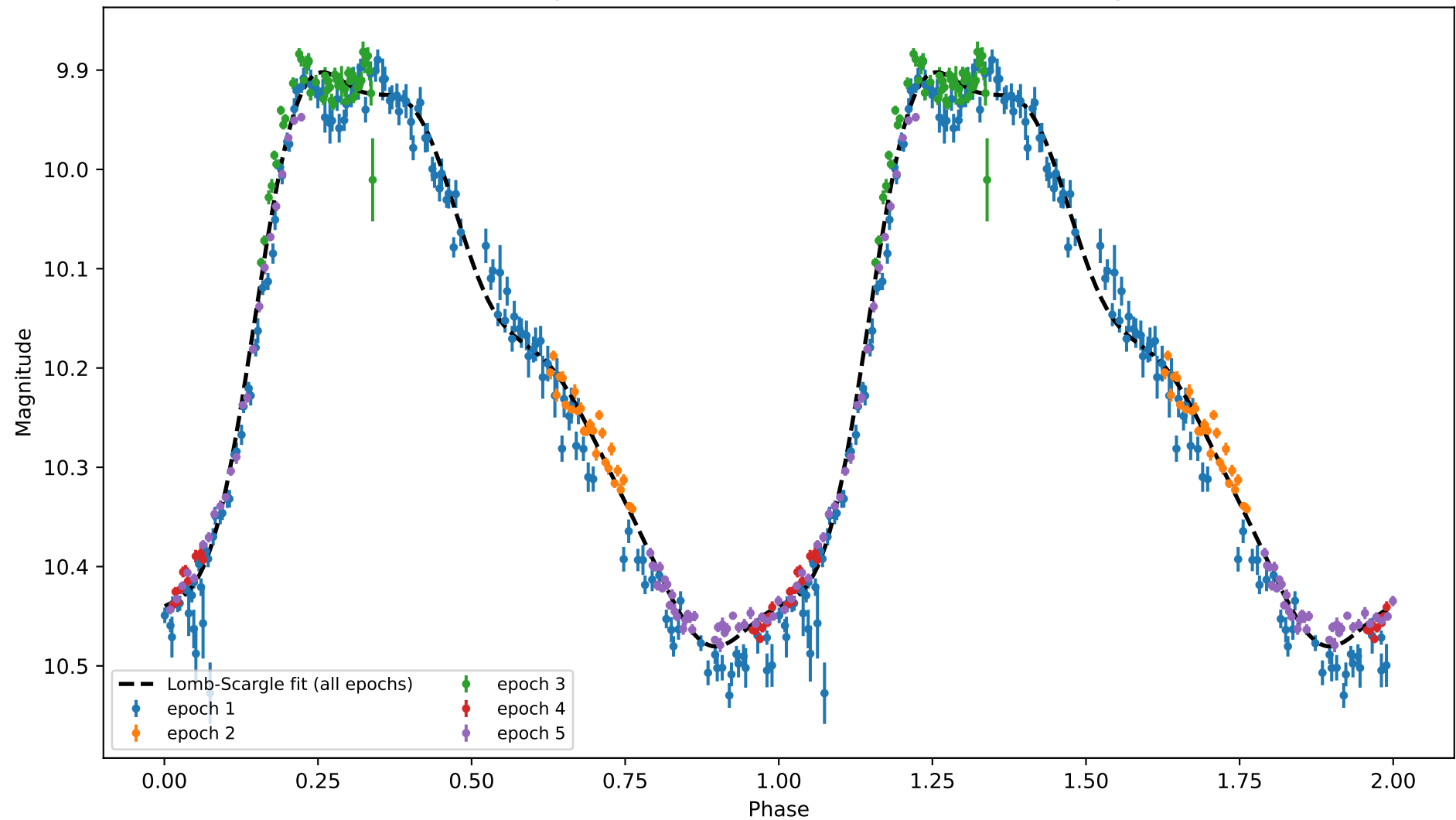
Lomb-Scargle Fit (nterms=5) - 0.3086298997995992 days
