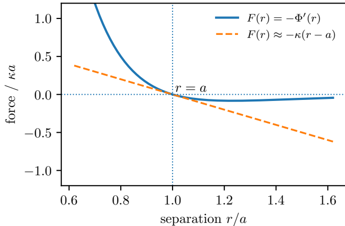
local linear restoring force
