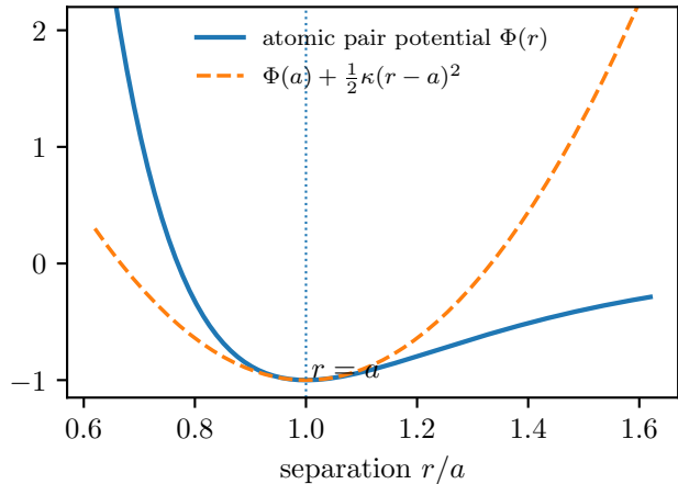
local quadratic approximation
