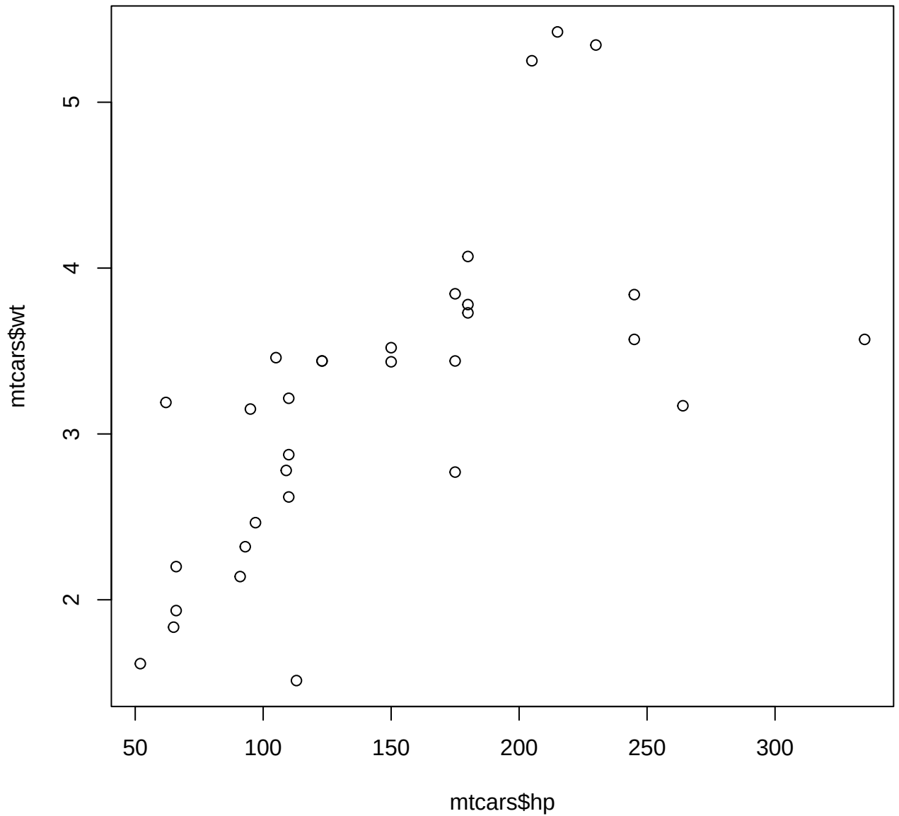
Scatter Plot HorsePower vs Weight
