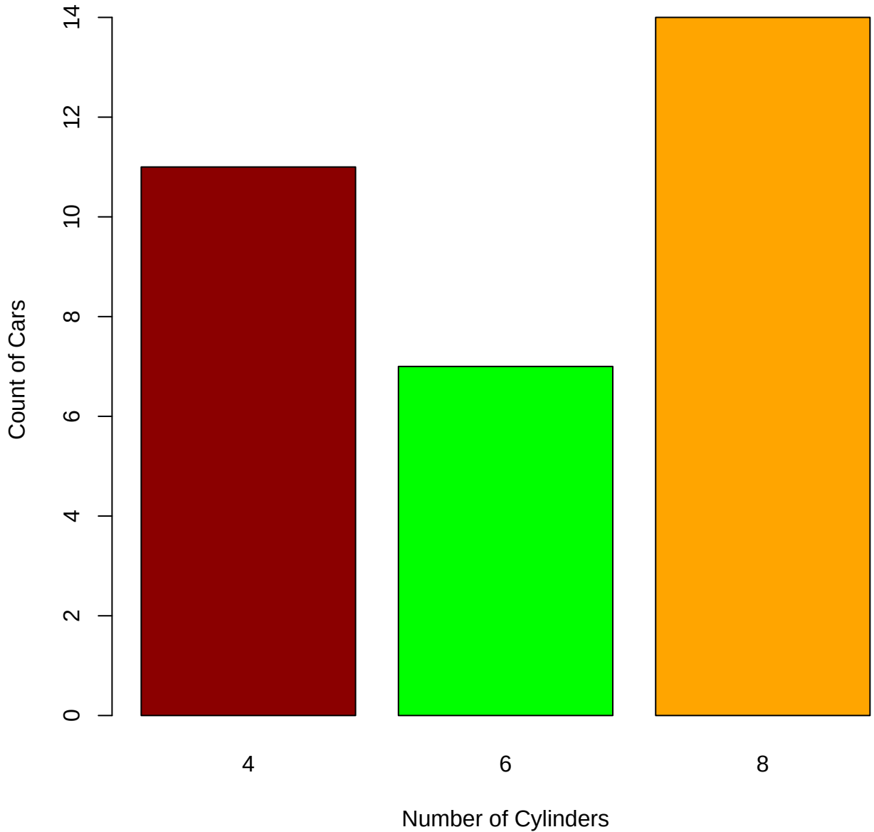
Count of Cars by Cylinder
