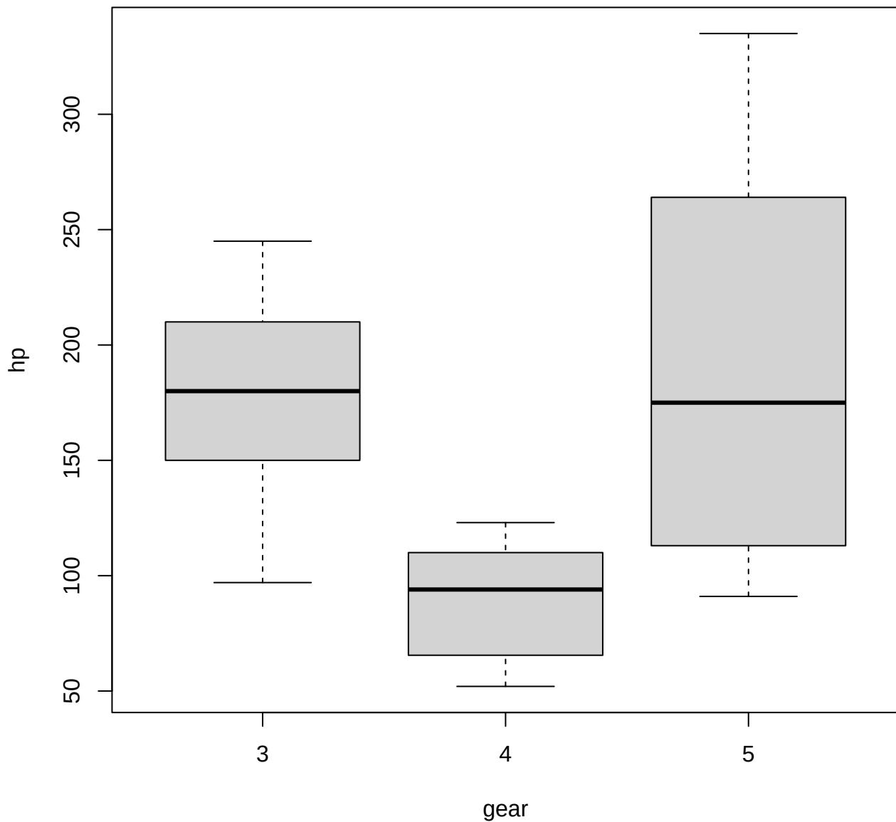
Boxplot of HorsePower vs Gear
