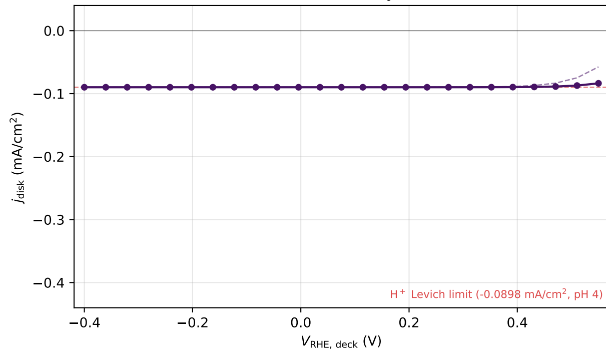
Total disk current density (deck axis)
