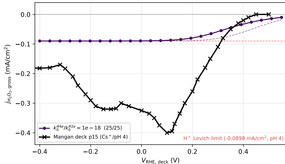
Gross \text{H}_2\text{O}_2 current (R2e channel) vs deck axis
