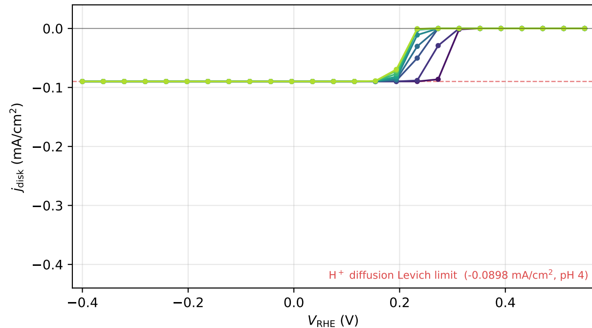
Total disk current density vs V_{\text{RHE}}
