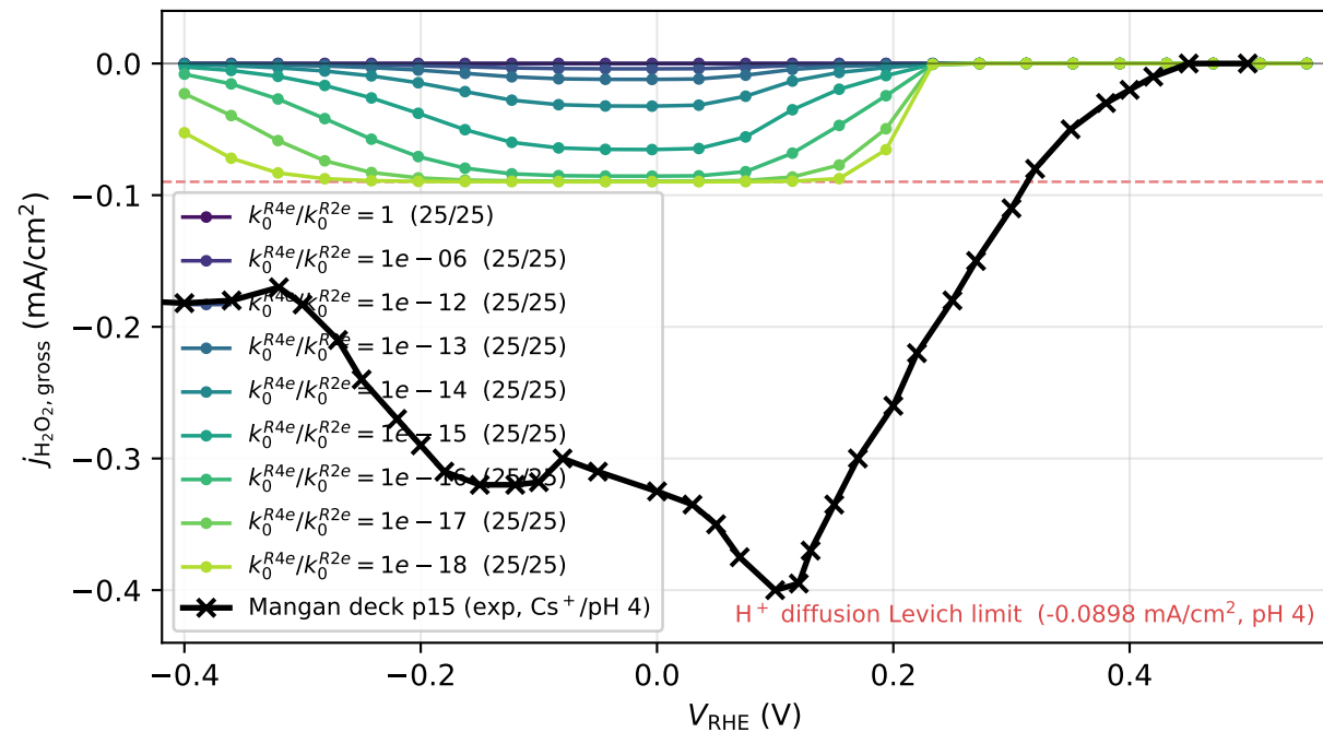
Gross \text{H}_2\text{O}_2 current (R2e channel) vs V_{\text{RHE}}
