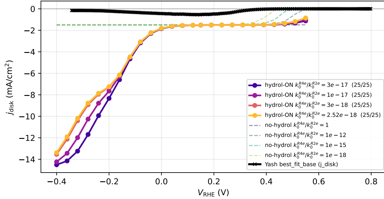
j_{\text{disk}} — full range
