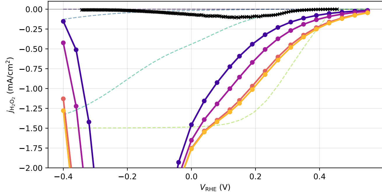
j_{\text{H}_2\text{O}_2} — zoomed to Yash range
