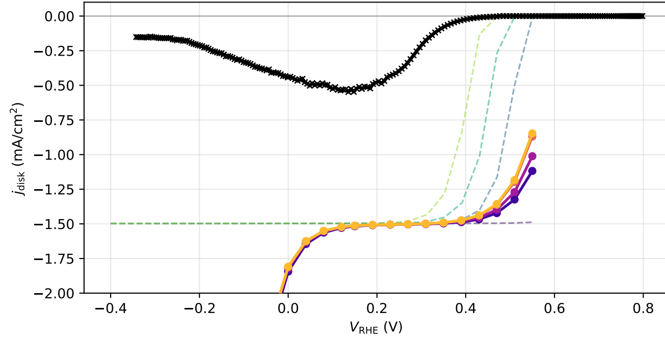
j_{\text{disk}} — zoomed to Yash range ( \pm 2\text{ mA/cm}^2 )
