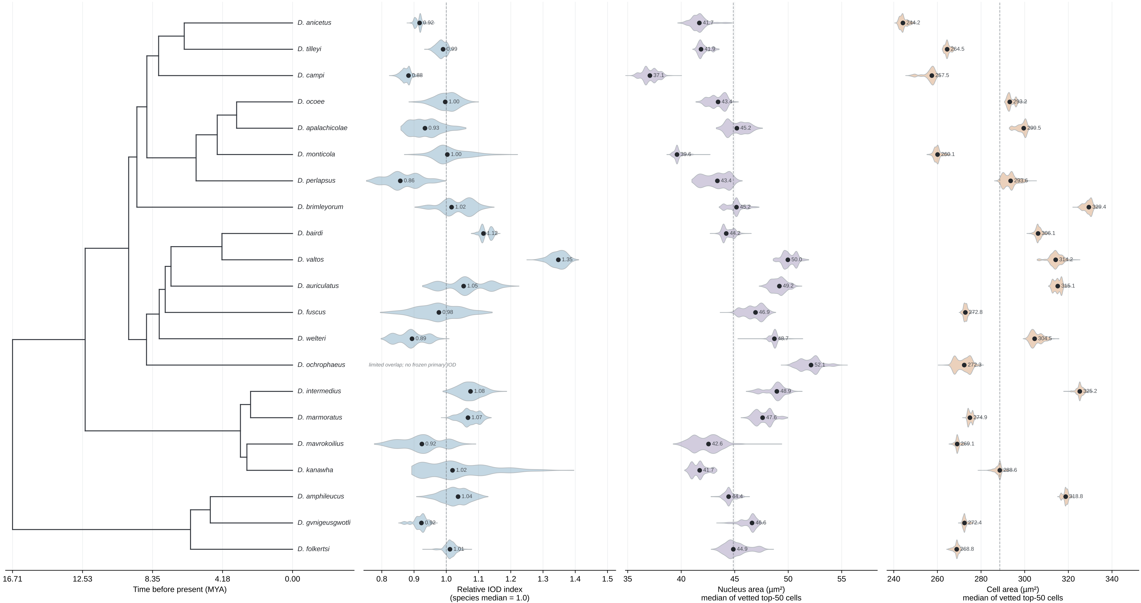
Time-calibrated phylogeny
