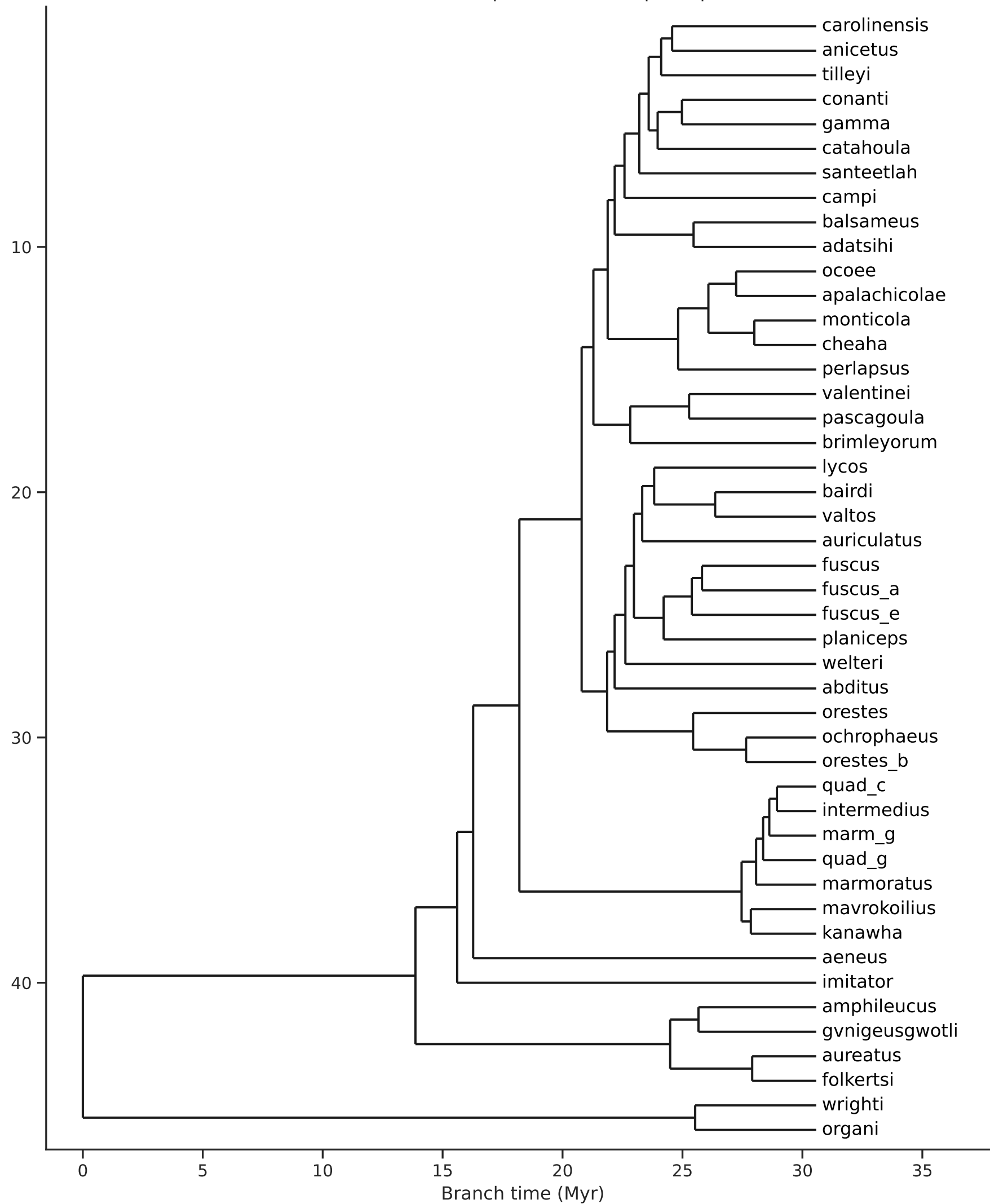
Source focal tree (46 tips; before exact panel prune)
