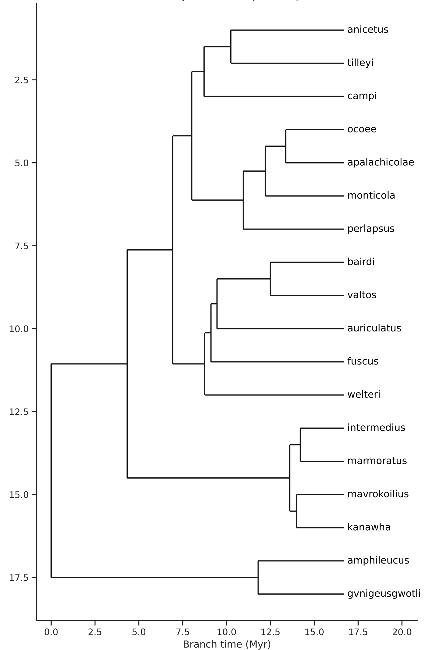
Frozen analysis tree (18 tips; after prune)
