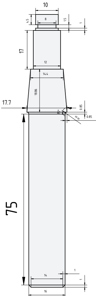
Dimension View
