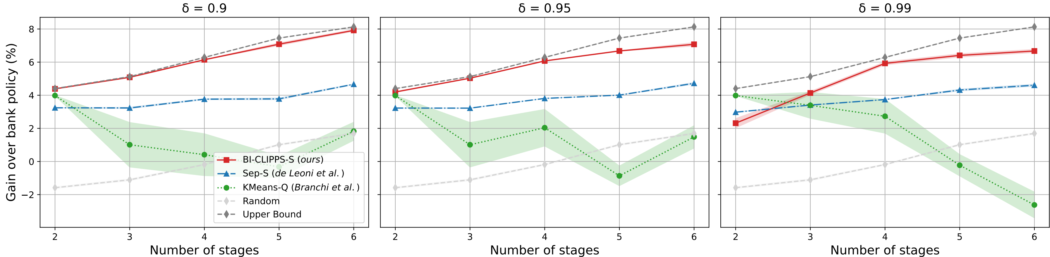
Performance across confounding levels for different numbers of stages
