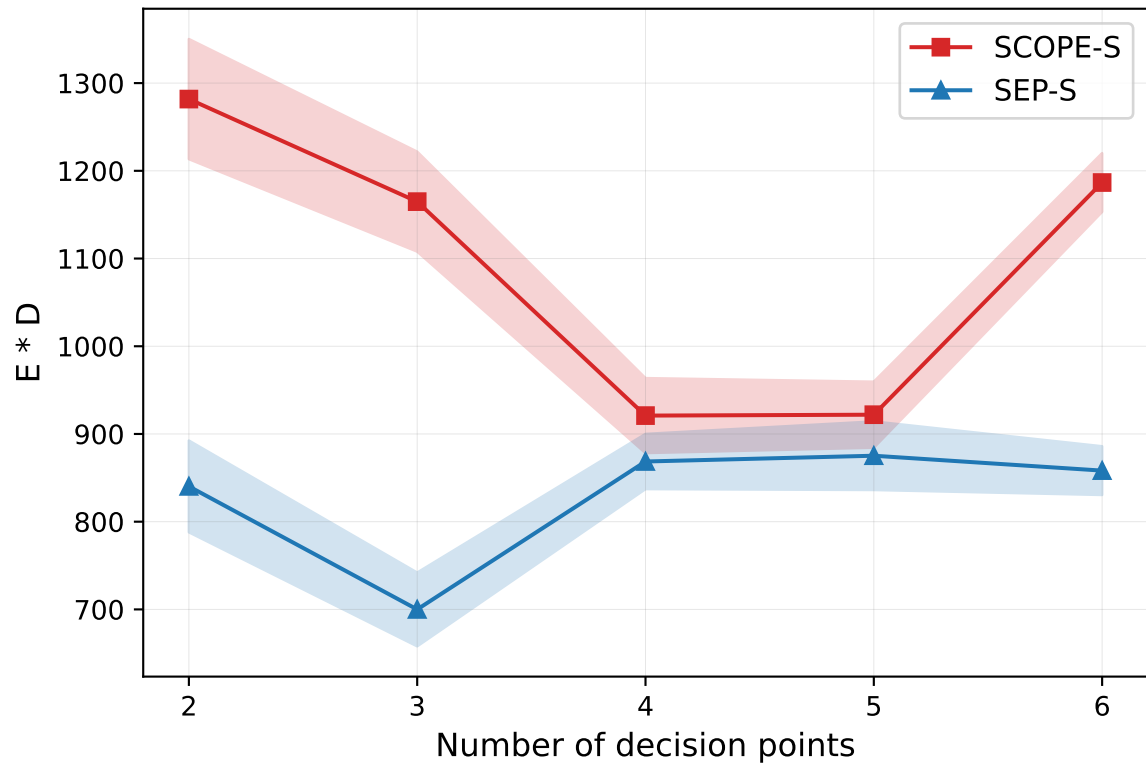
SimBPIC17 (train size = 10K)
