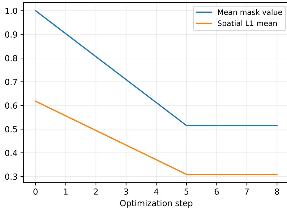
Local sparsity penalties
