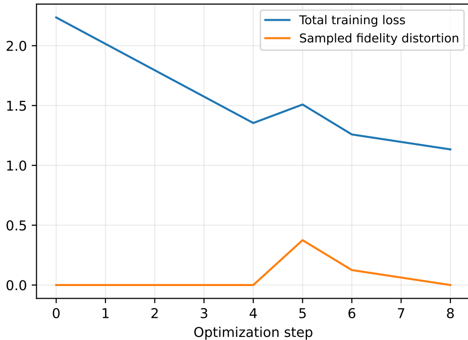
Noisy training estimates
