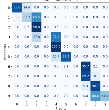
MQ
