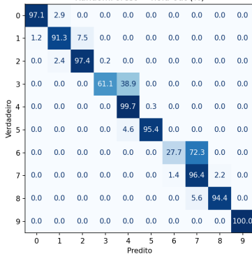
Random Forest
