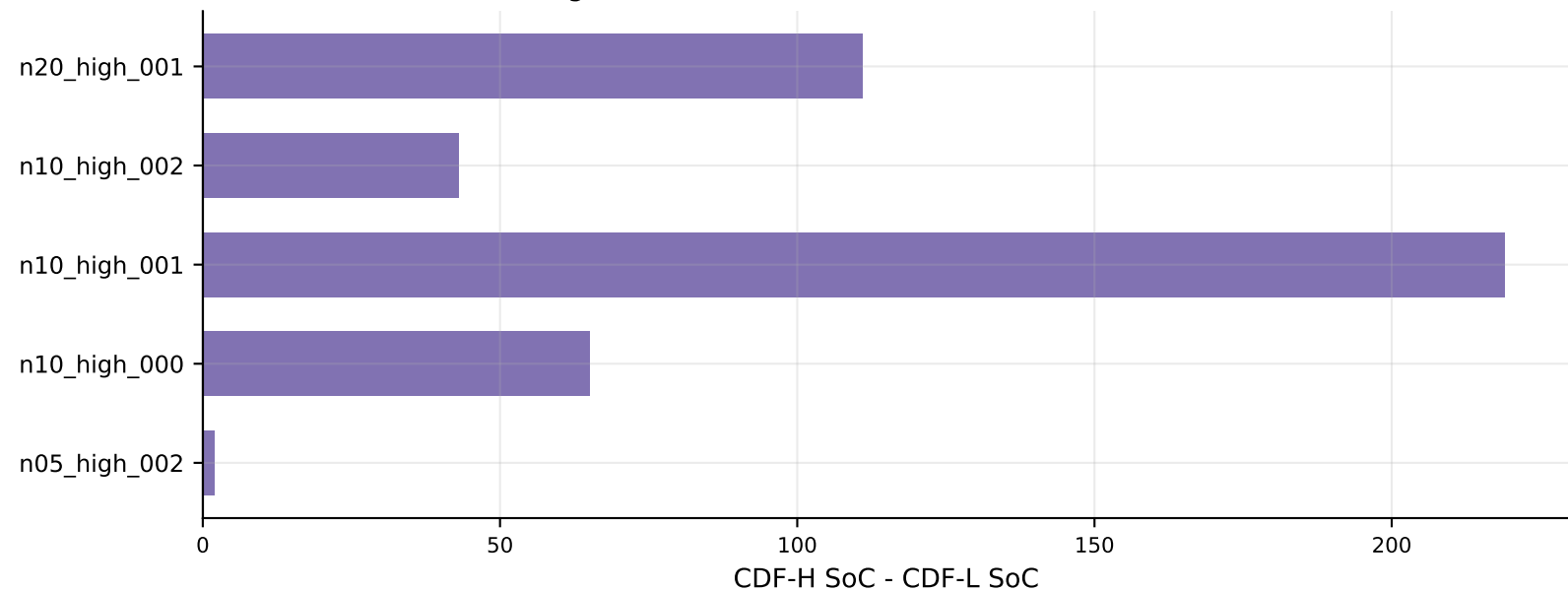
CDF-H vs CDF-L direction test on differing instances Negative = CDF-H better; Positive = CDF-L better
