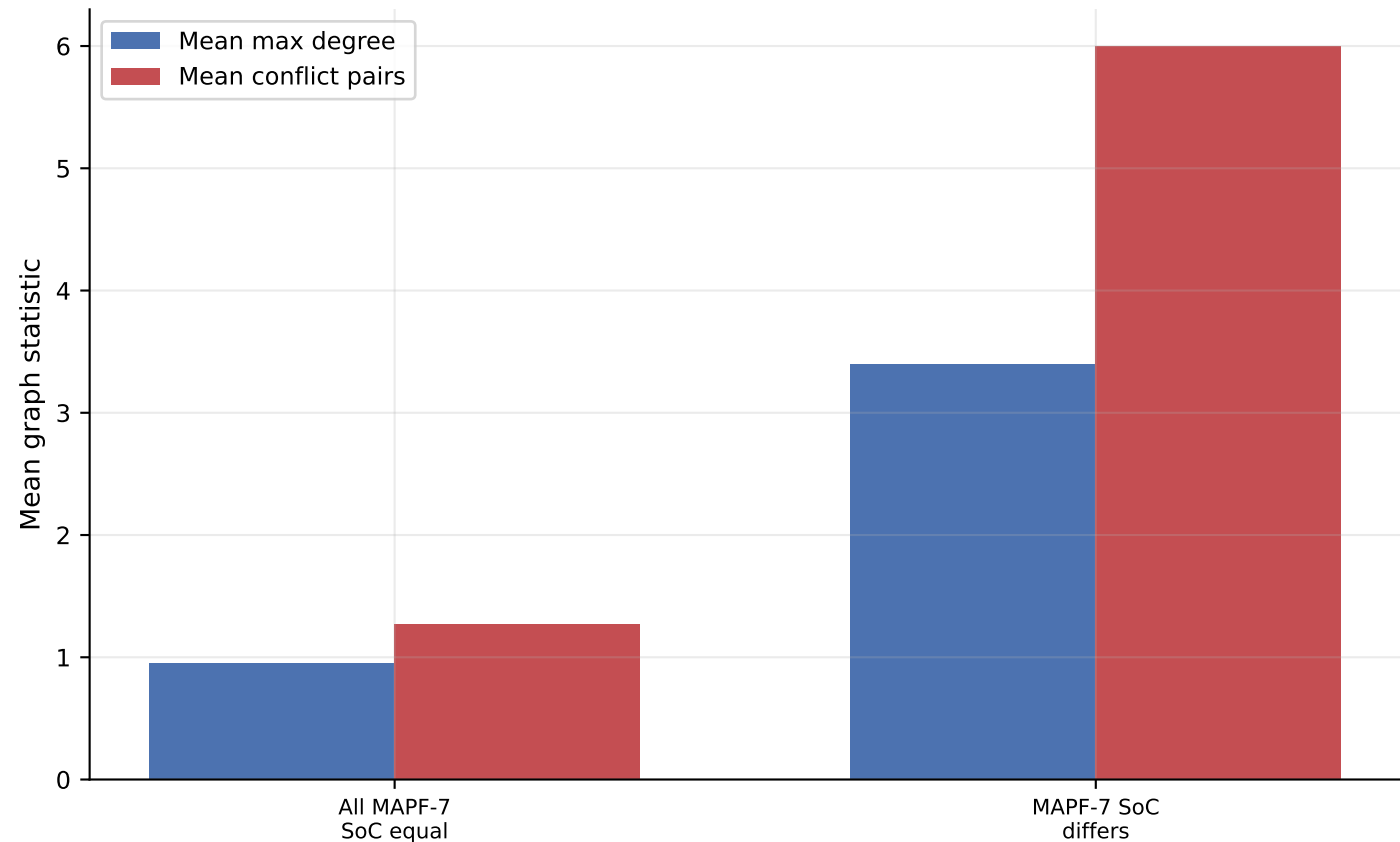
Conflict-graph structure vs MAPF-7 priority sensitivity (descriptive; not causal; n equal=22, differ=5)
