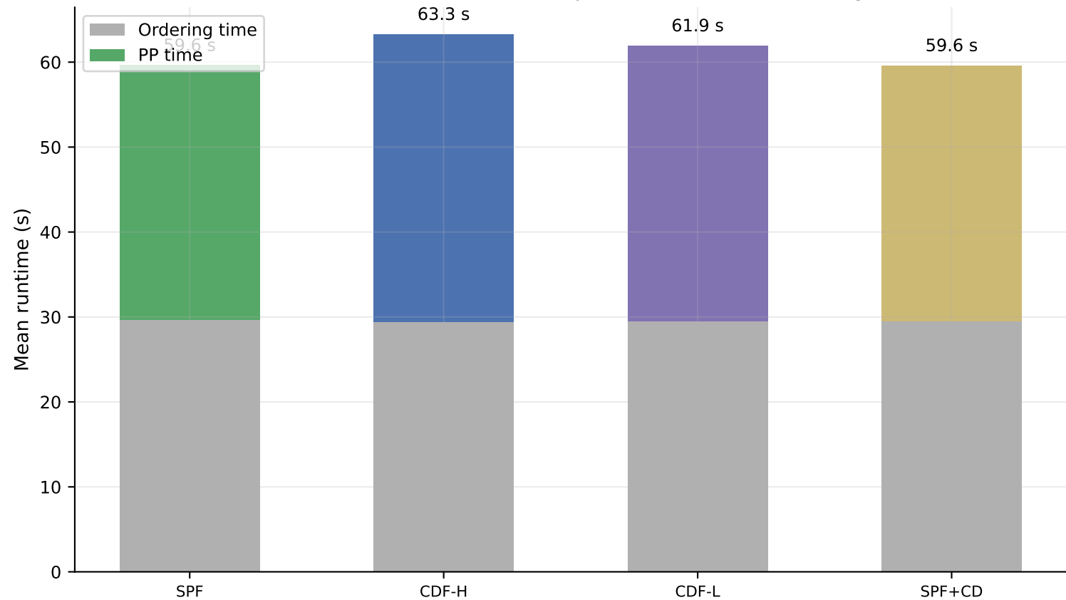
Mean runtime composition (SPF from MAPF-6; MAPF-7 from separate run; total = ordering + PP)
