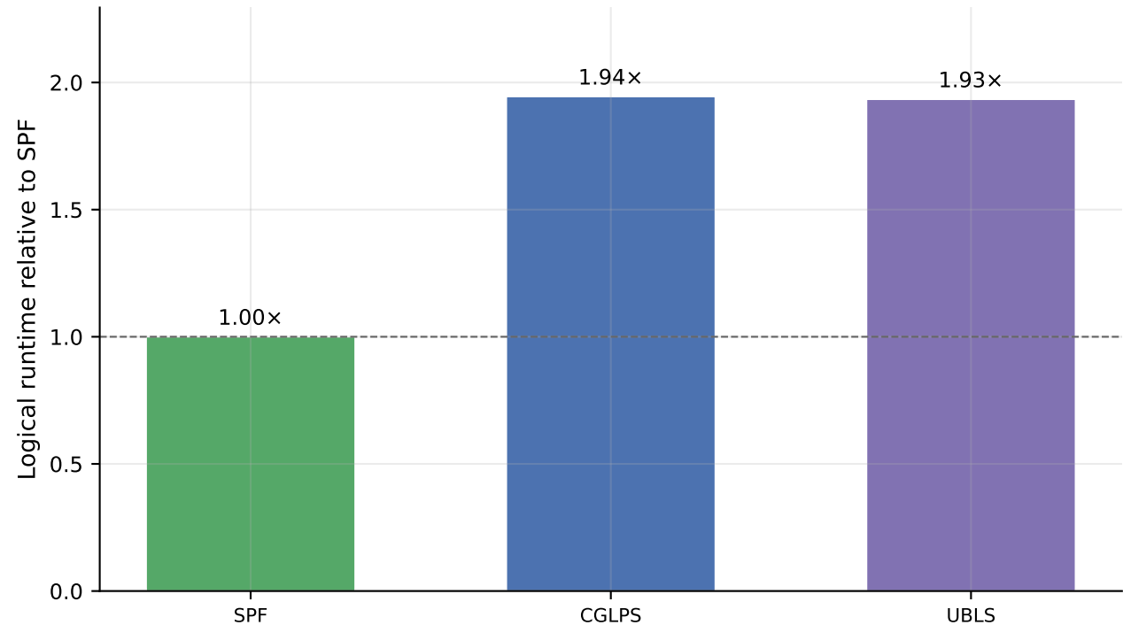
Cost of bounded search (pooled logical runtime)
