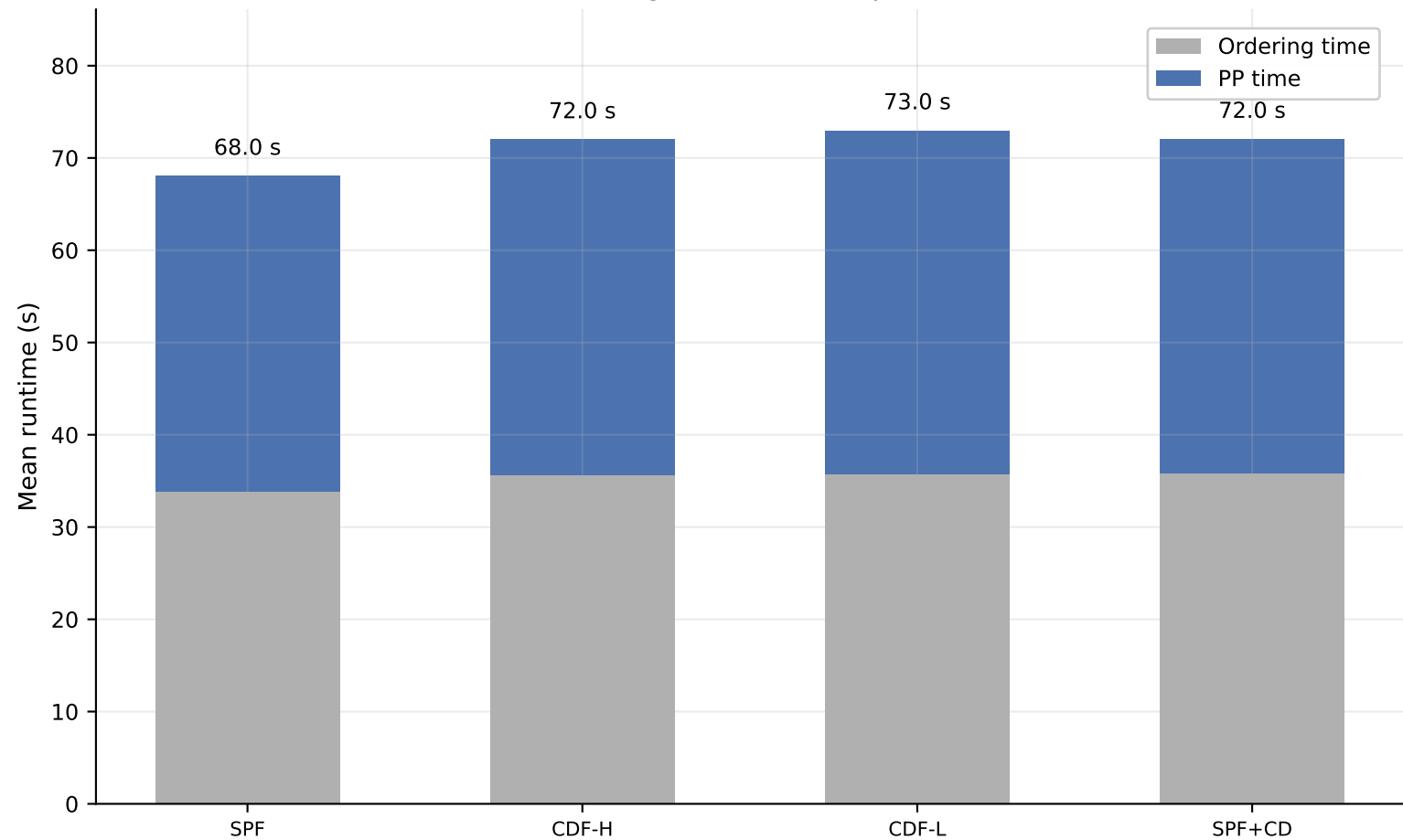
Held-out runtime composition (total = ordering + PP from independent runs)
