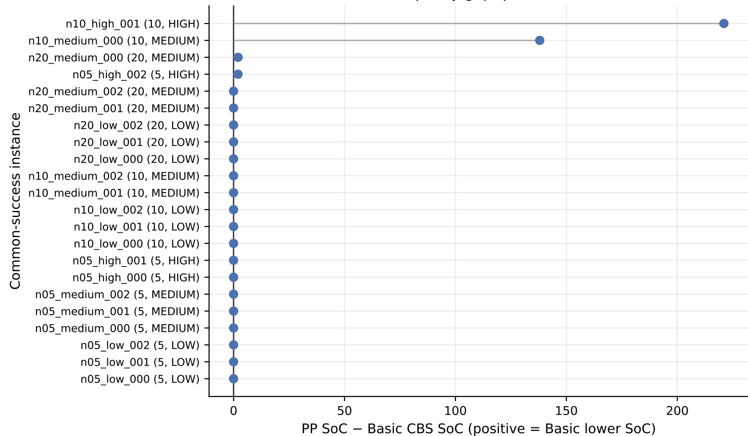
PP vs Basic CBS solution-quality gap (paired common-success cases)
