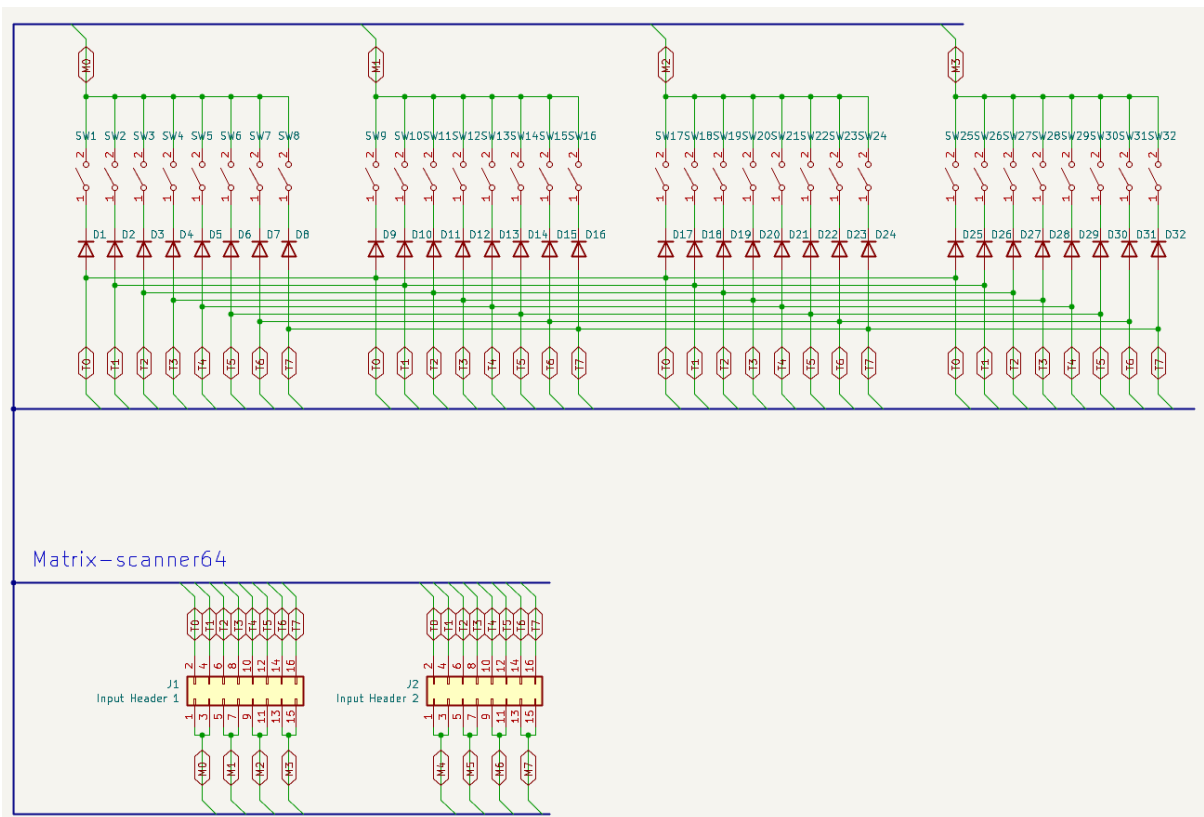
Figure 4: Diode matrix wiring diagram
