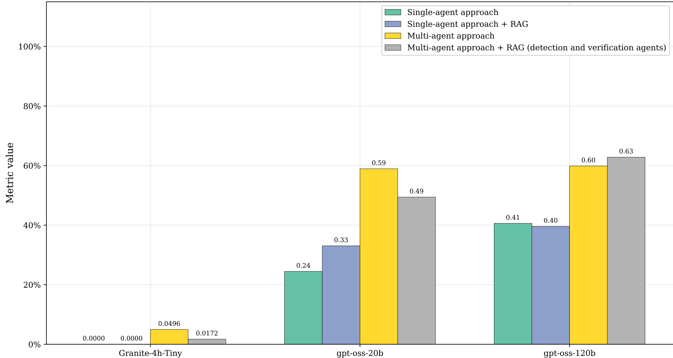
Comparison of F1 across selected large language models and the single-agent and multi-agent approaches
