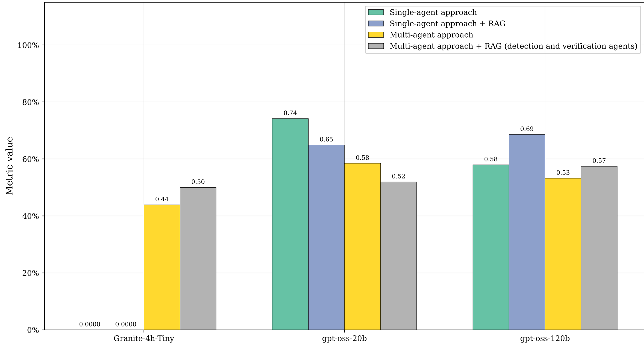
Comparison of Precision across selected large language models and the single-agent and multi-agent approaches
