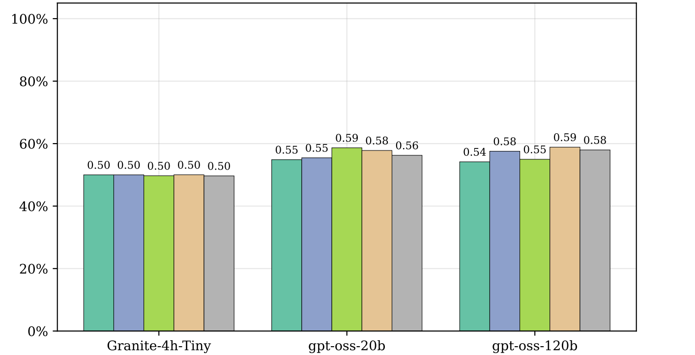
Comparison of Balanced Accuracy across selected large language models and the single-agent and multi-agent approaches
