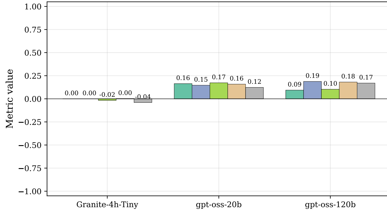
Comparison of MCC across selected large language models and the single-agent and multi-agent approaches
