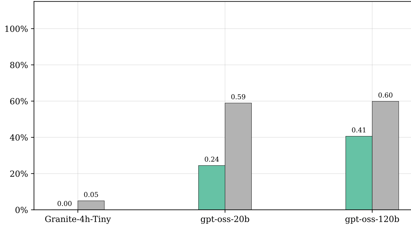
Comparison of F1 across selected large language models and the single-agent and multi-agent approaches
