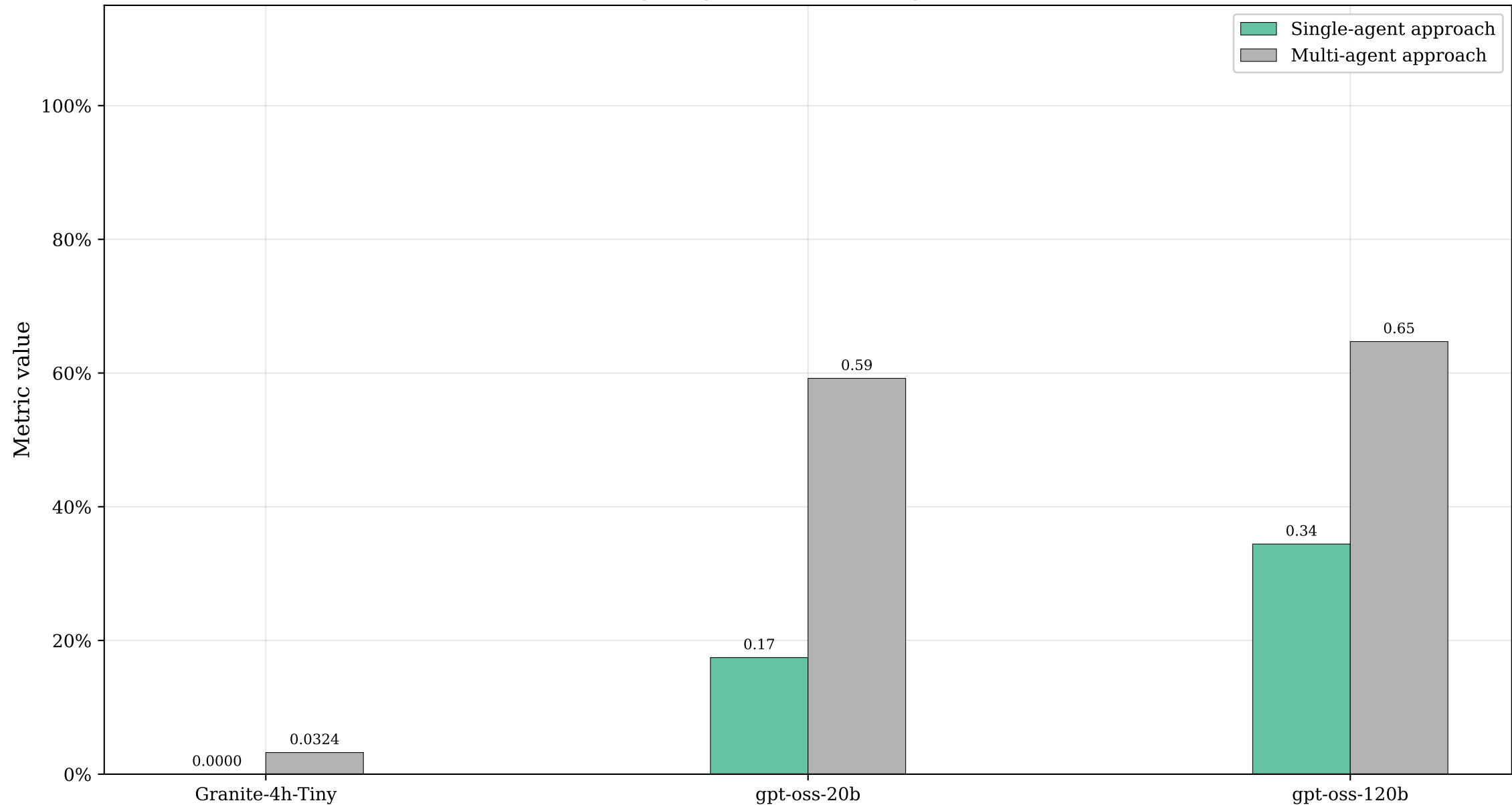
Comparison of F2 across selected large language models and the single-agent and multi-agent approaches
