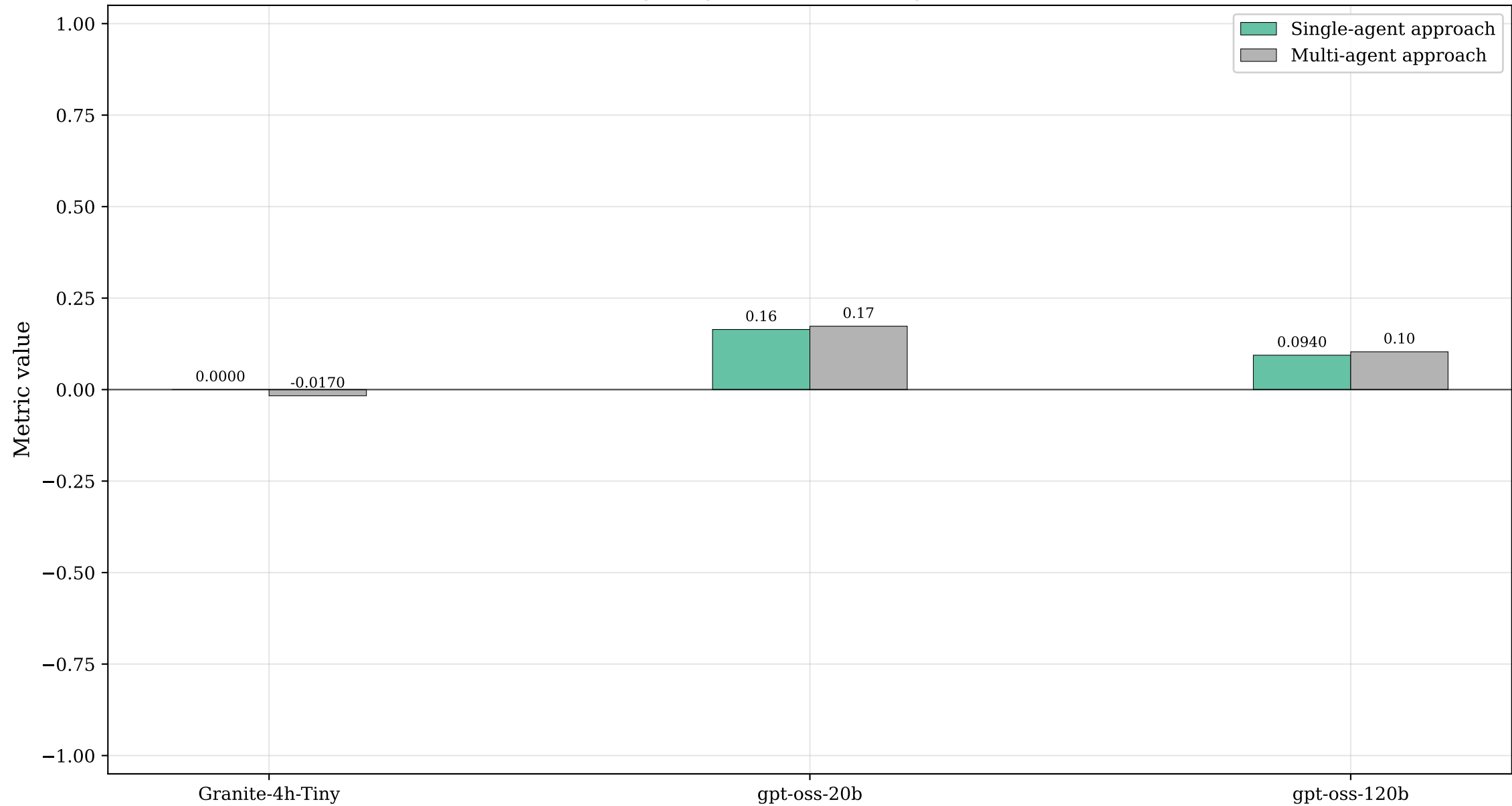
Comparison of MCC across selected large language models and the single-agent and multi-agent approaches
