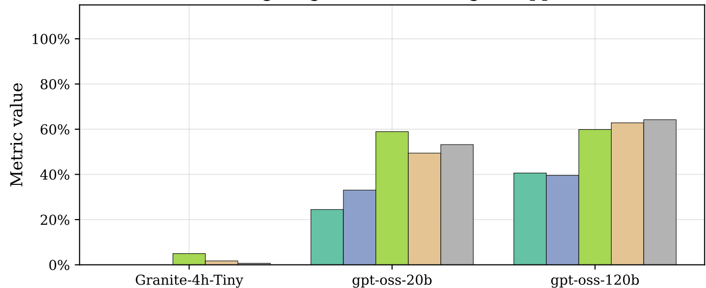
Comparison of F1 across selected large language models and the single-agent and multi-agent approaches
