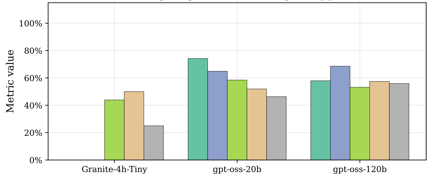
Comparison of Precision across selected large language models and the single-agent and multi-agent approaches
