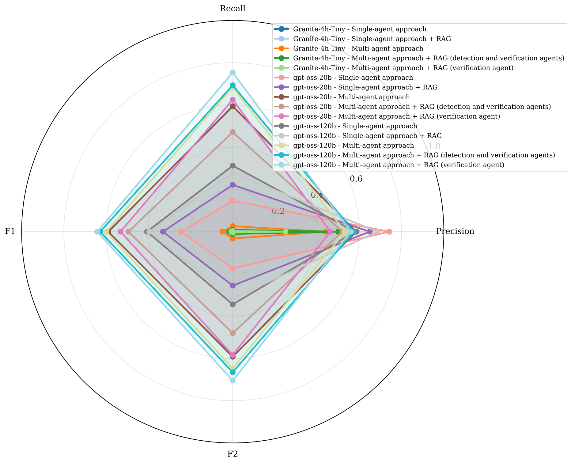
Comparison of Recall, Precision, F1, and F2 across selected large language models and the single-agent and multi-agent approaches
